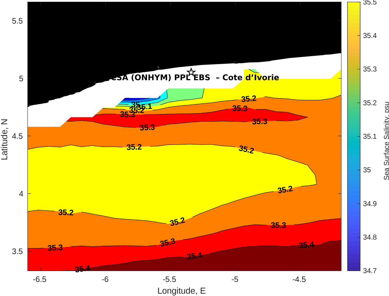
Surface Salinity for CSA (ONHYM) PPL EBS - Cote d'Ivoire at 09-Aug-2025 00:00:00
