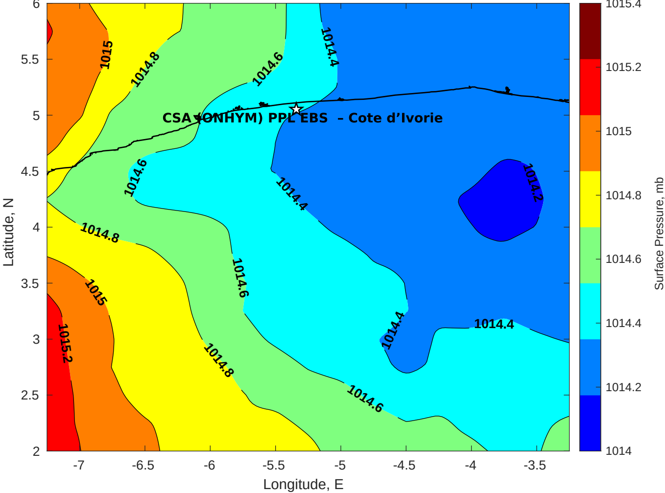
Surface Pressure (mb) for CSA (ONHYM) PPL EBS - Cote d'Ivoire at 10-Aug-2025 00:00:00
