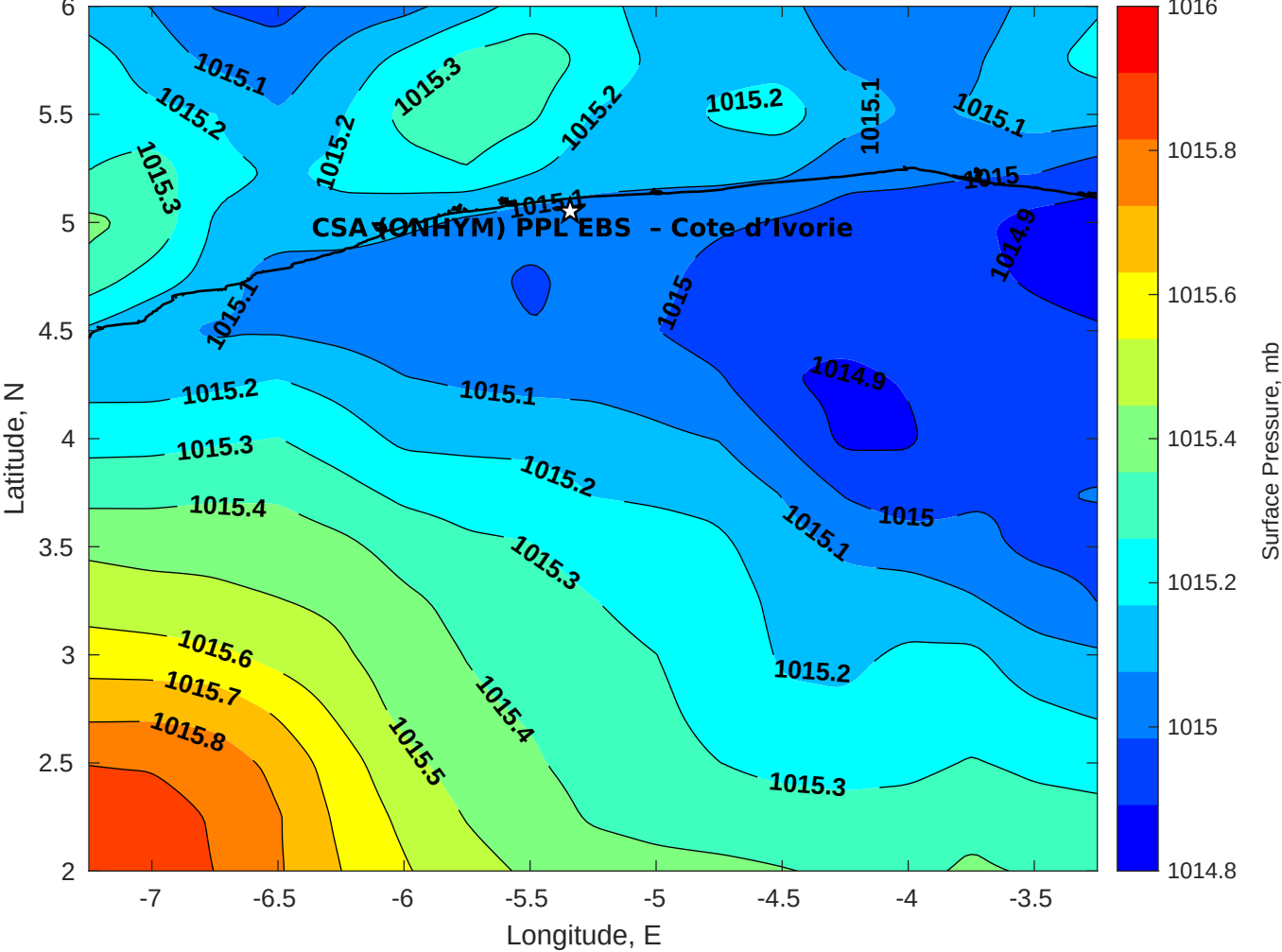
Surface Pressure (mb) for CSA (ONHYM) PPL EBS - Cote d'Ivoire at 12-Aug-2025 00:00:00
