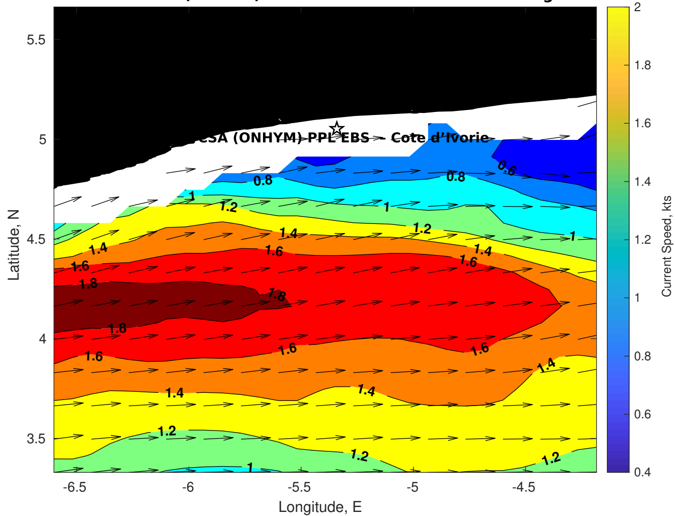
Surface Currents for CSA (ONHYM) PPL EBS - Cote d'Ivoire at 09-Aug-2025 00:00:00
