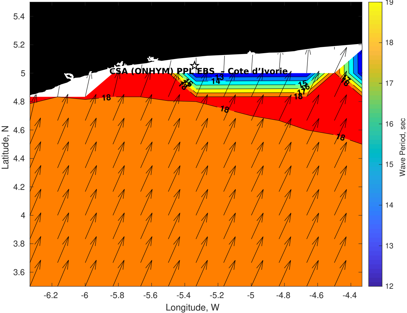
Wave Period (sec) for CSA (ONHYM) PPL EBS - Cote d'Ivoire at 10-Aug-2025 09:00:00
