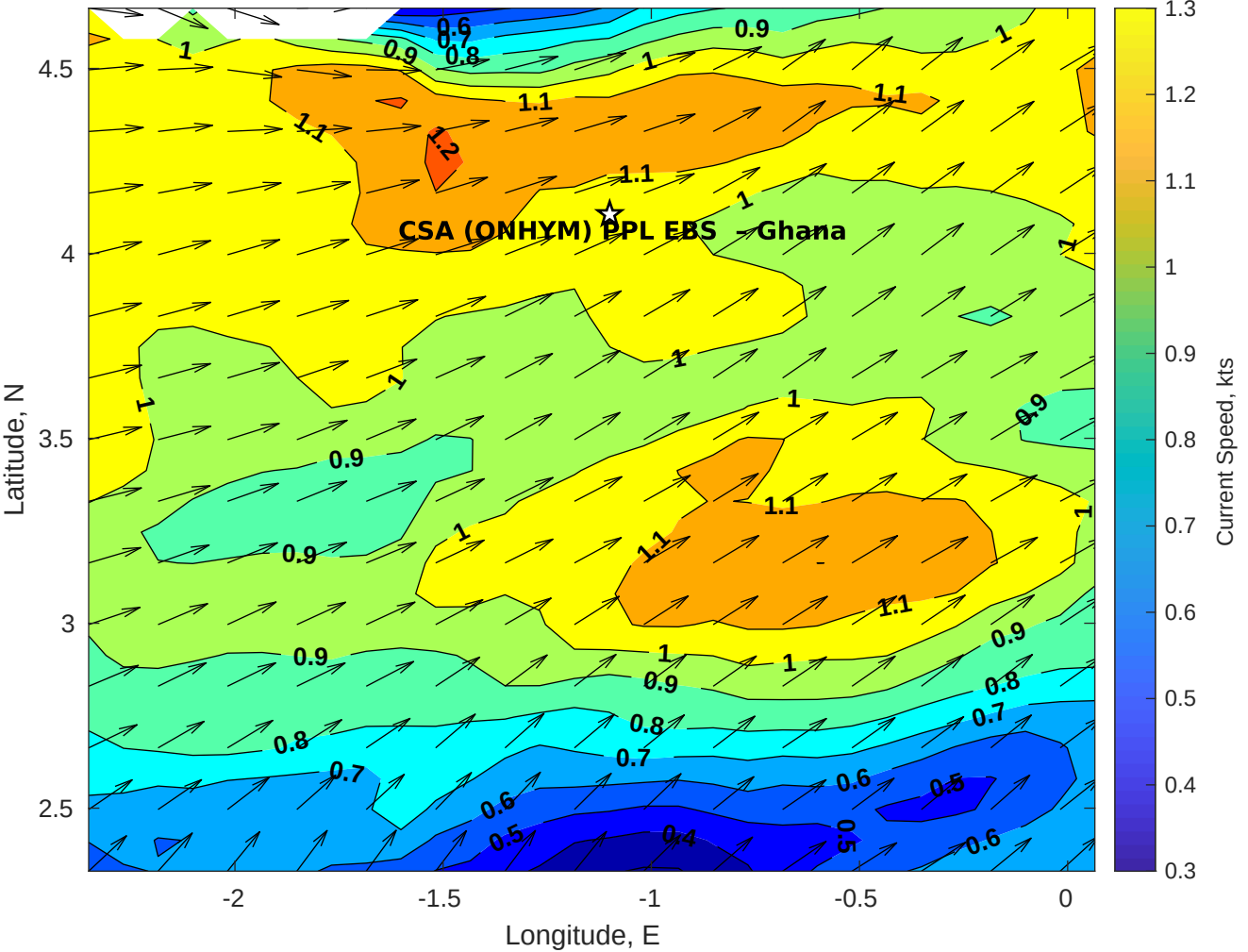
Surface Currents for CSA (ONHYM) PPL EBS - Ghana at 09-Aug-2025 00:00:00
