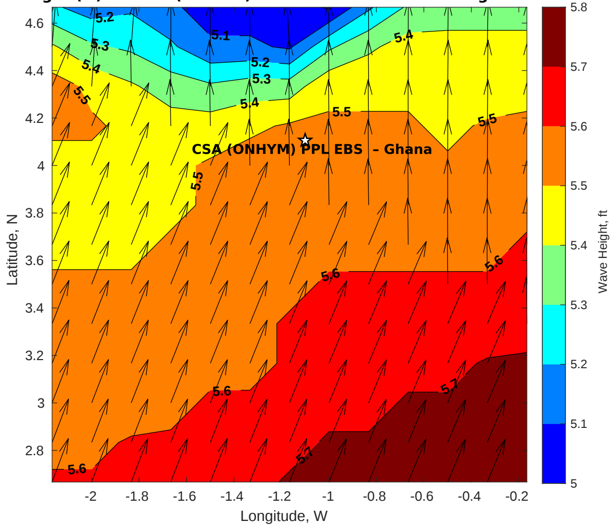
Wave Height (ft) for CSA (ONHYM) PPL EBS - Ghana at 10-Aug-2025 09:00:00
