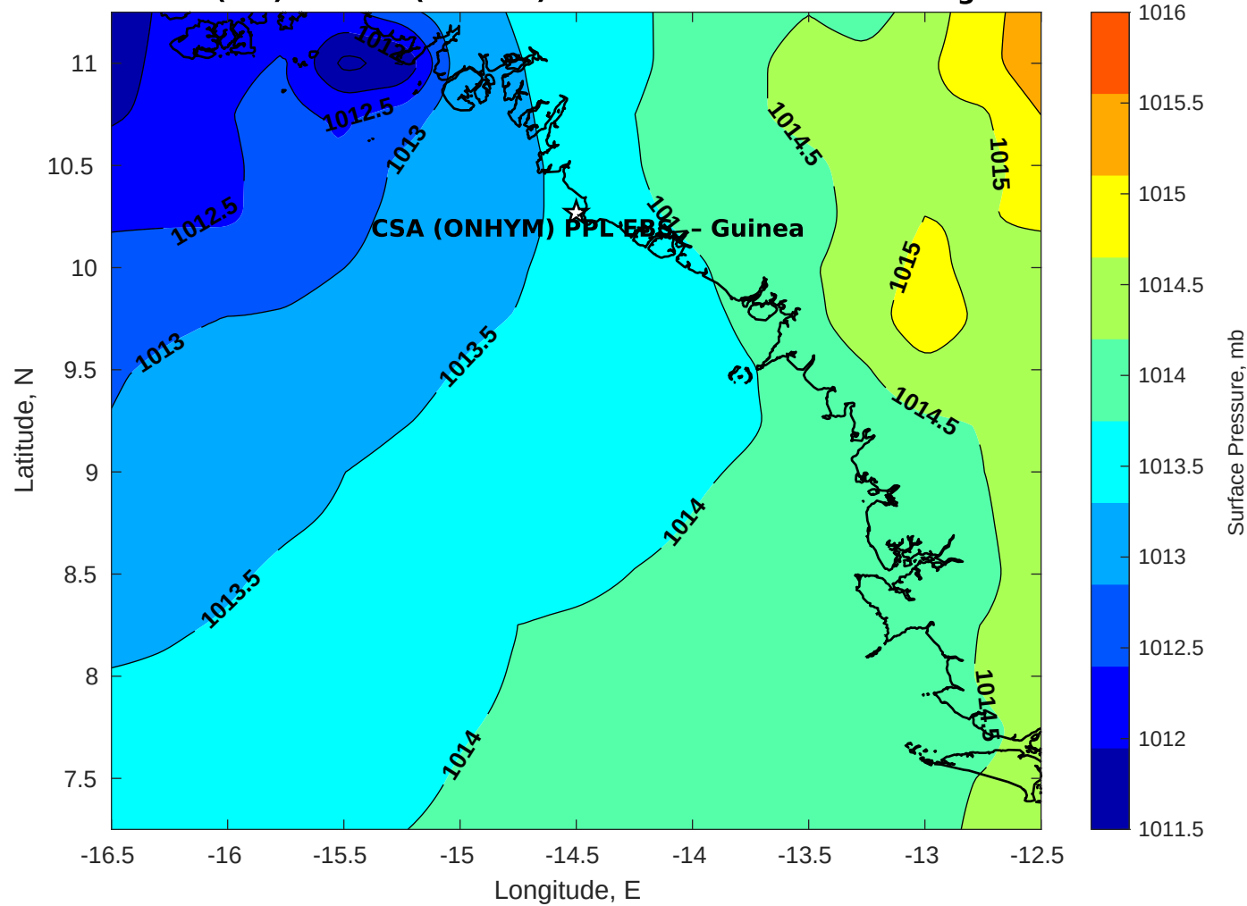
Surface Pressure (mb) for CSA (ONHYM) PPL EBS - Guinea at 10-Aug-2025 00:00:00
