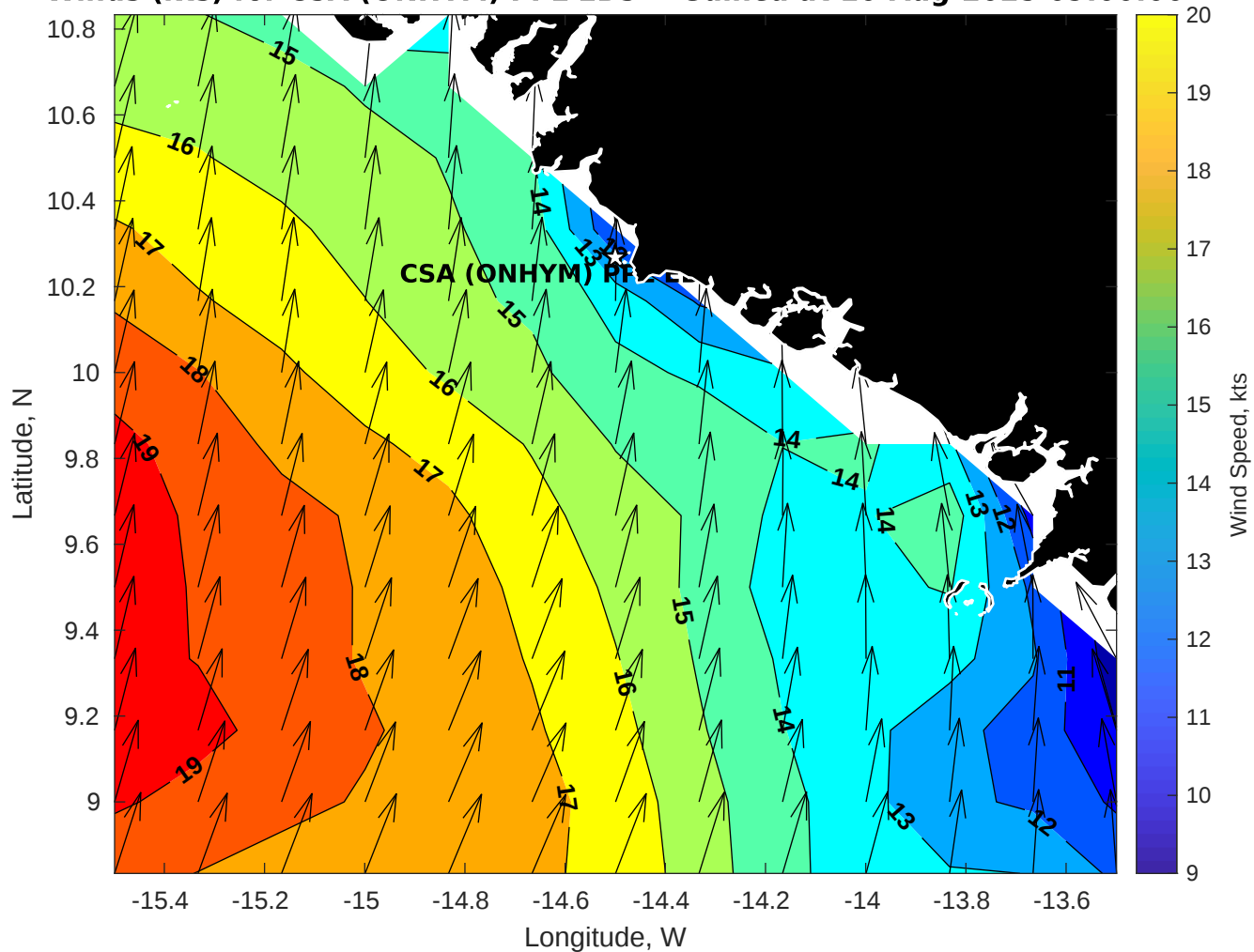
Winds (kts) for CSA (ONHYM) PPL EBS - Guinea at 10-Aug-2025 09:00:00
