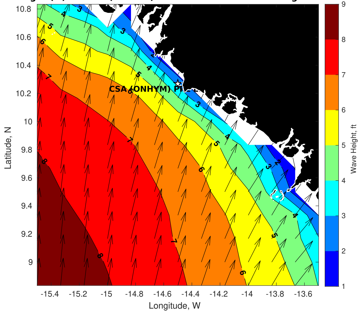
Wave Height (ft) for CSA (ONHYM) PPL EBS - Guinea at 10-Aug-2025 09:00:00
