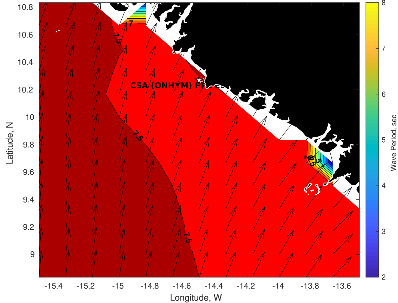
Wave Period (sec) for CSA (ONHYM) PPL EBS - Guinea at 10-Aug-2025 09:00:00
