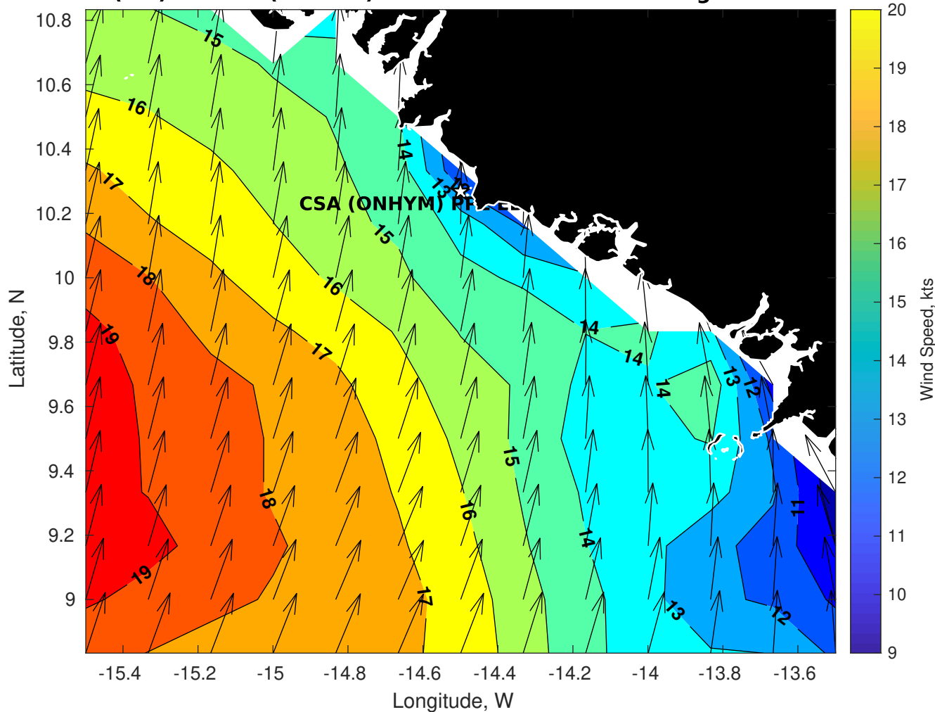
Winds (kts) for CSA (ONHYM) PPL EBS - Guinea at 10-Aug-2025 09:00:00
