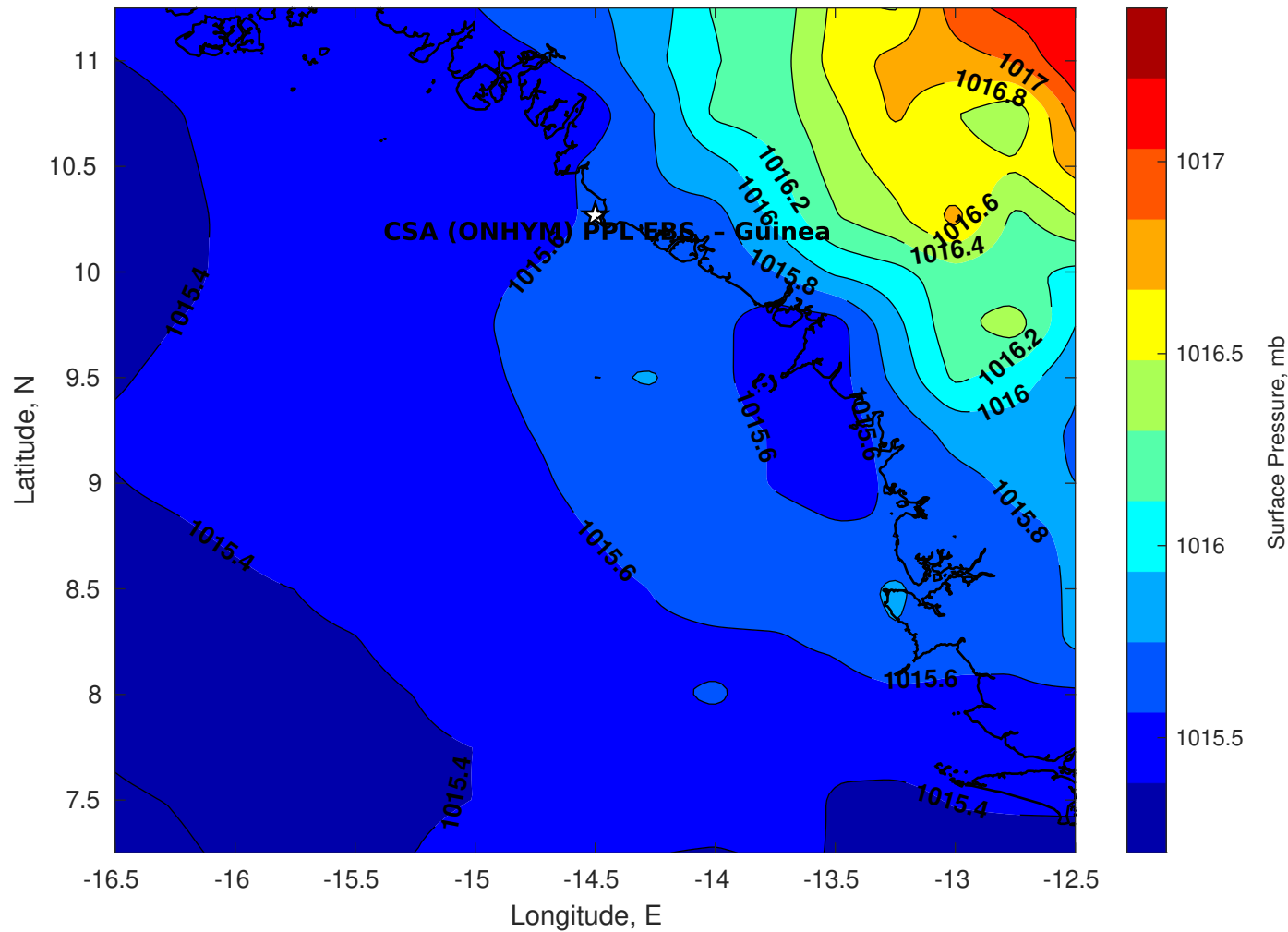
Surface Pressure (mb) for CSA (ONHYM) PPL EBS - Guinea at 11-Aug-2025 00:00:00
