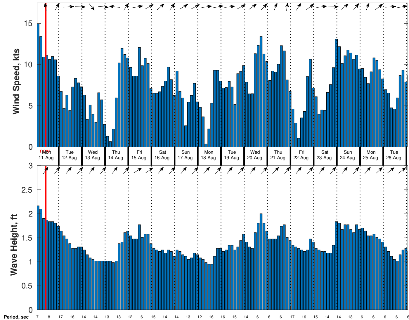
Wind & Wave Forecast for CSA (ONHYM) PPL EBS - Guinea from 10-Aug-2025 01:00:00 to 26-Aug-2025 01:00:00
