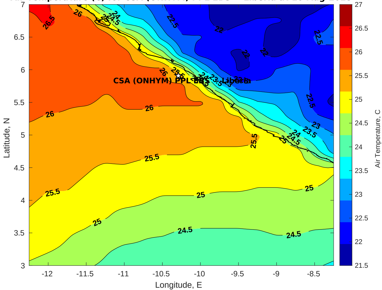
Air Temperature (C) for CSA (ONHYM) PPL EBS - Liberia at 10-Aug-2025
