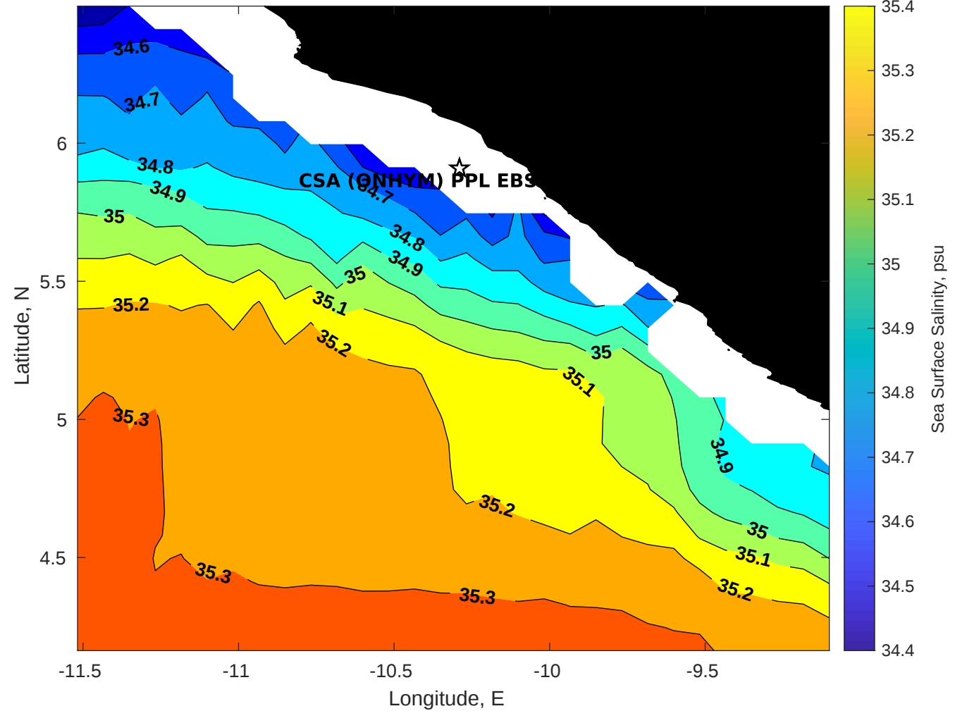
Surface Salinity for CSA (ONHYM) PPL EBS - Liberia at 09-Aug-2025 00:00:00
