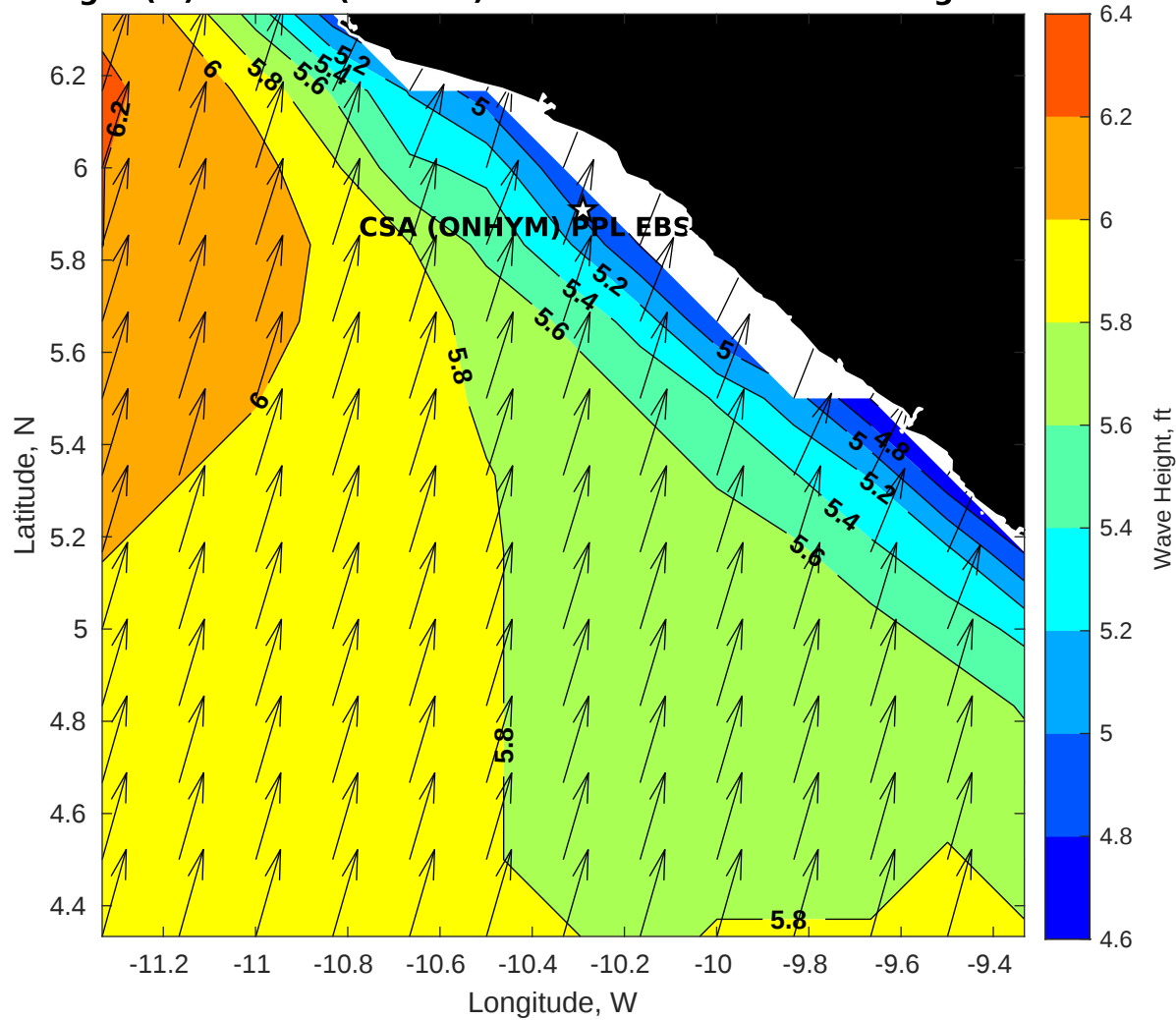
Wave Height (ft) for CSA (ONHYM) PPL EBS - Liberia at 10-Aug-2025 09:00:00
