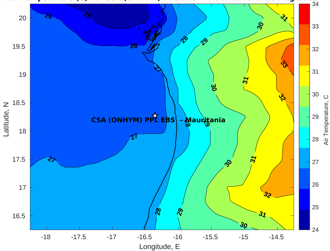
Air Temperature (C) for CSA (ONHYM) PPL EBS - Mauritania at 10-Aug-2025
