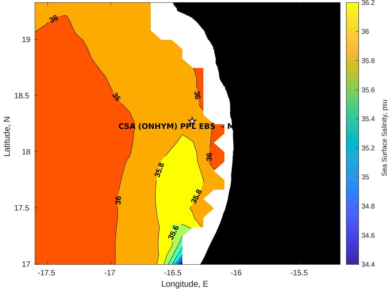
Surface Salinity for CSA (ONHYM) PPL EBS - Mauritania at 09-Aug-2025 00:00:00
