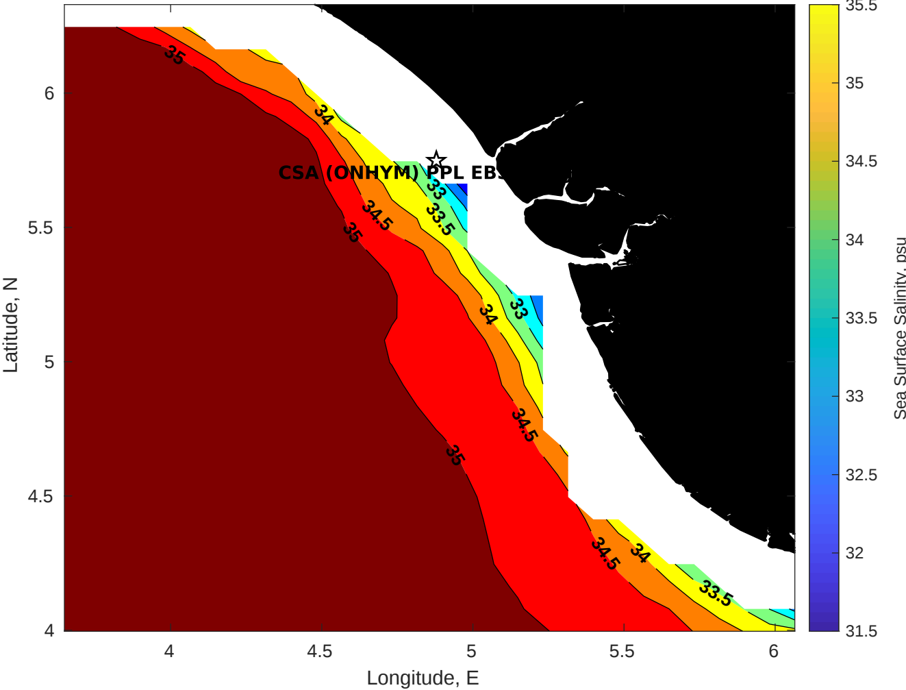
Surface Salinity for CSA (ONHYM) PPL EBS - Nigeria at 09-Aug-2025 00:00:00
