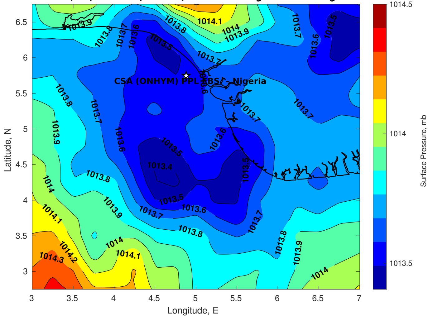
Surface Pressure (mb) for CSA (ONHYM) PPL EBS - Nigeria at 10-Aug-2025 00:00:00
