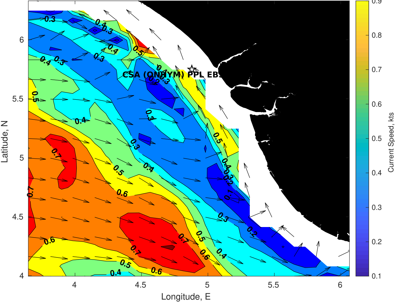
Surface Currents for CSA (ONHYM) PPL EBS - Nigeria at 09-Aug-2025 00:00:00
