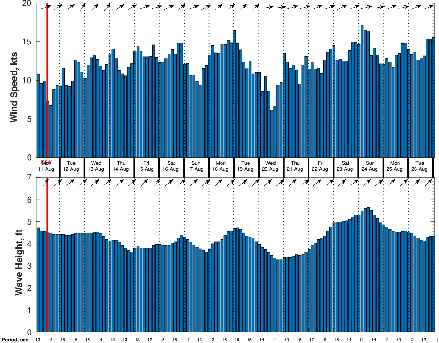
Wind & Wave Forecast for CSA (ONHYM) PPL EBS - Nigeria from 10-Aug-2025 02:00:00 to 26-Aug-2025 02:00:00
