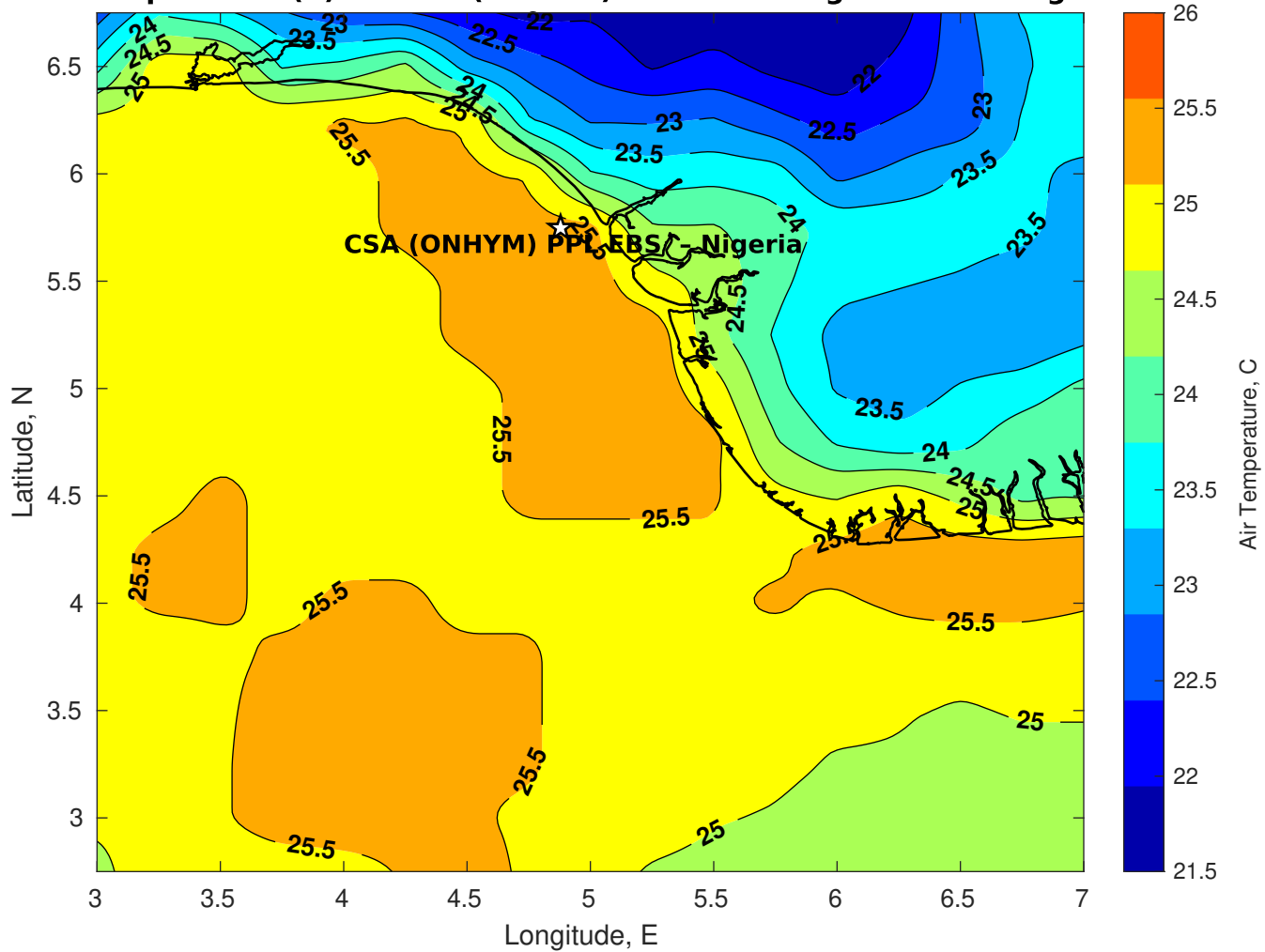
Air Temperature (C) for CSA (ONHYM) PPL EBS - Nigeria at 10-Aug-2025
