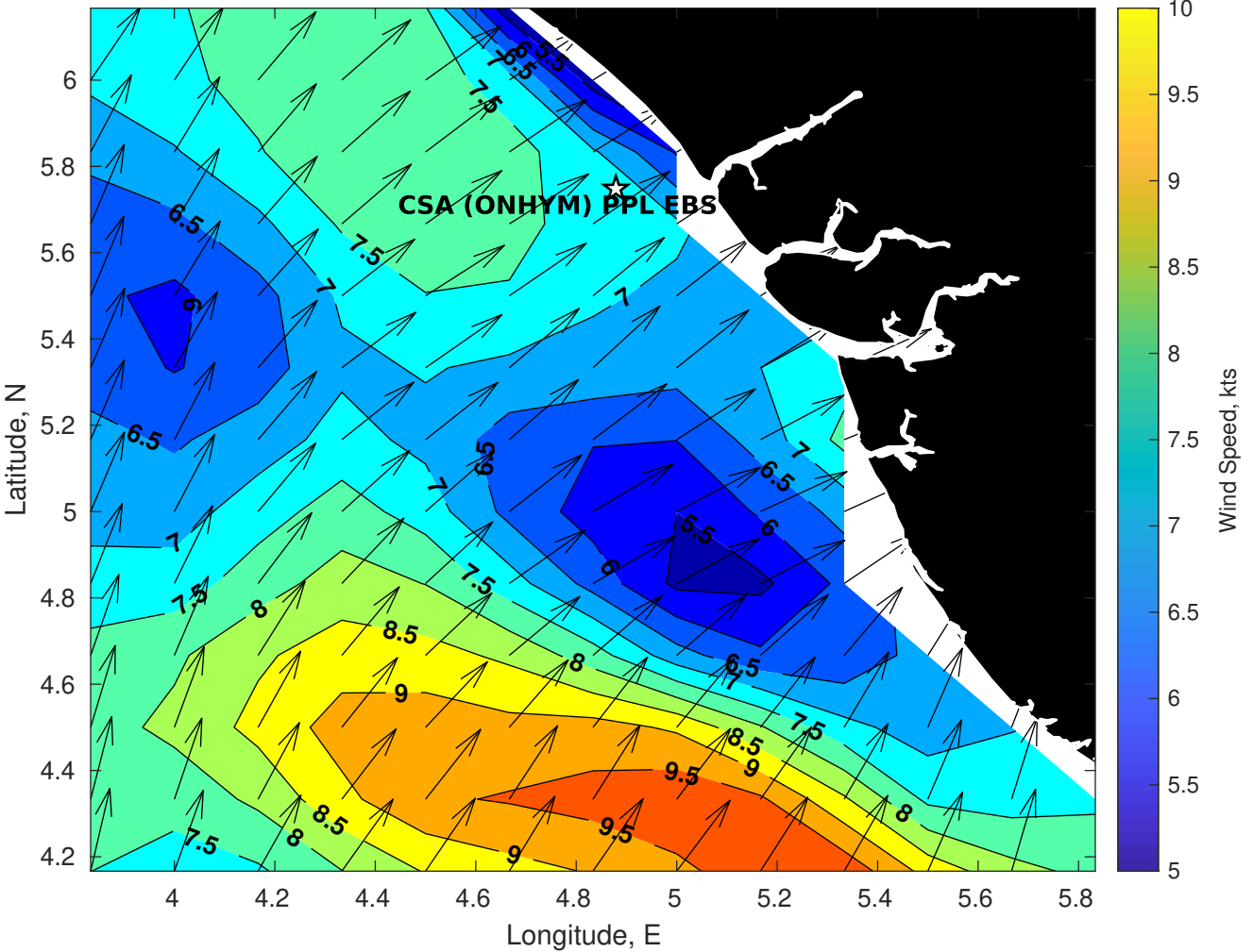
Winds (kts) for CSA (ONHYM) PPL EBS - Nigeria at 10-Aug-2025 09:00:00
