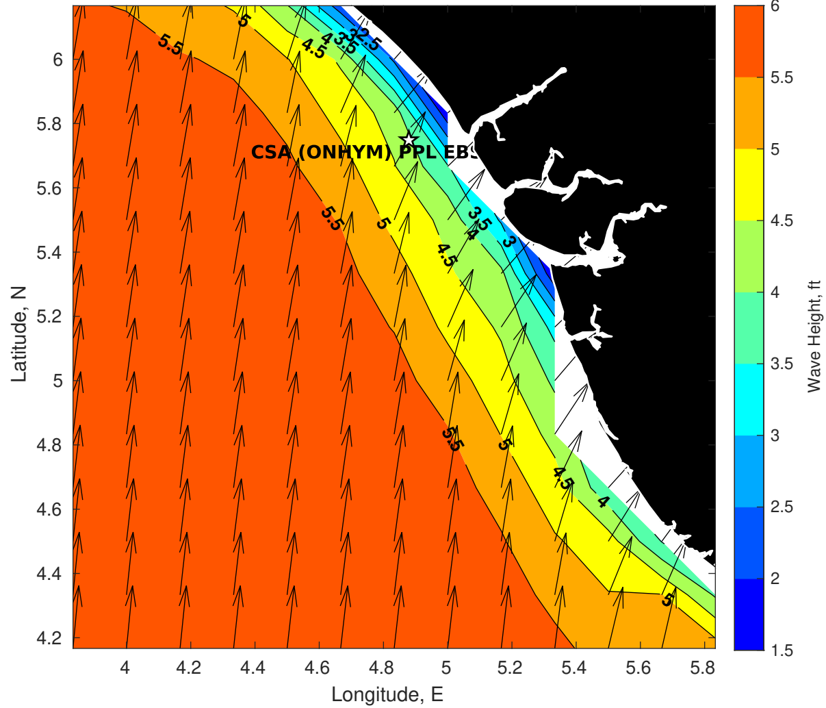
Wave Height (ft) for CSA (ONHYM) PPL EBS - Nigeria at 10-Aug-2025 09:00:00
