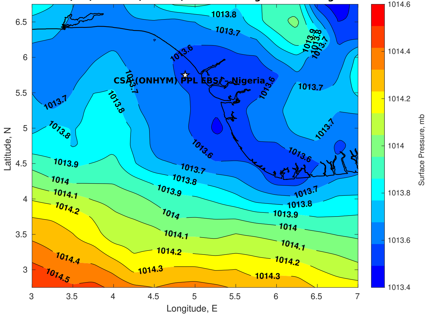
Surface Pressure (mb) for CSA (ONHYM) PPL EBS - Nigeria at 11-Aug-2025 00:00:00
