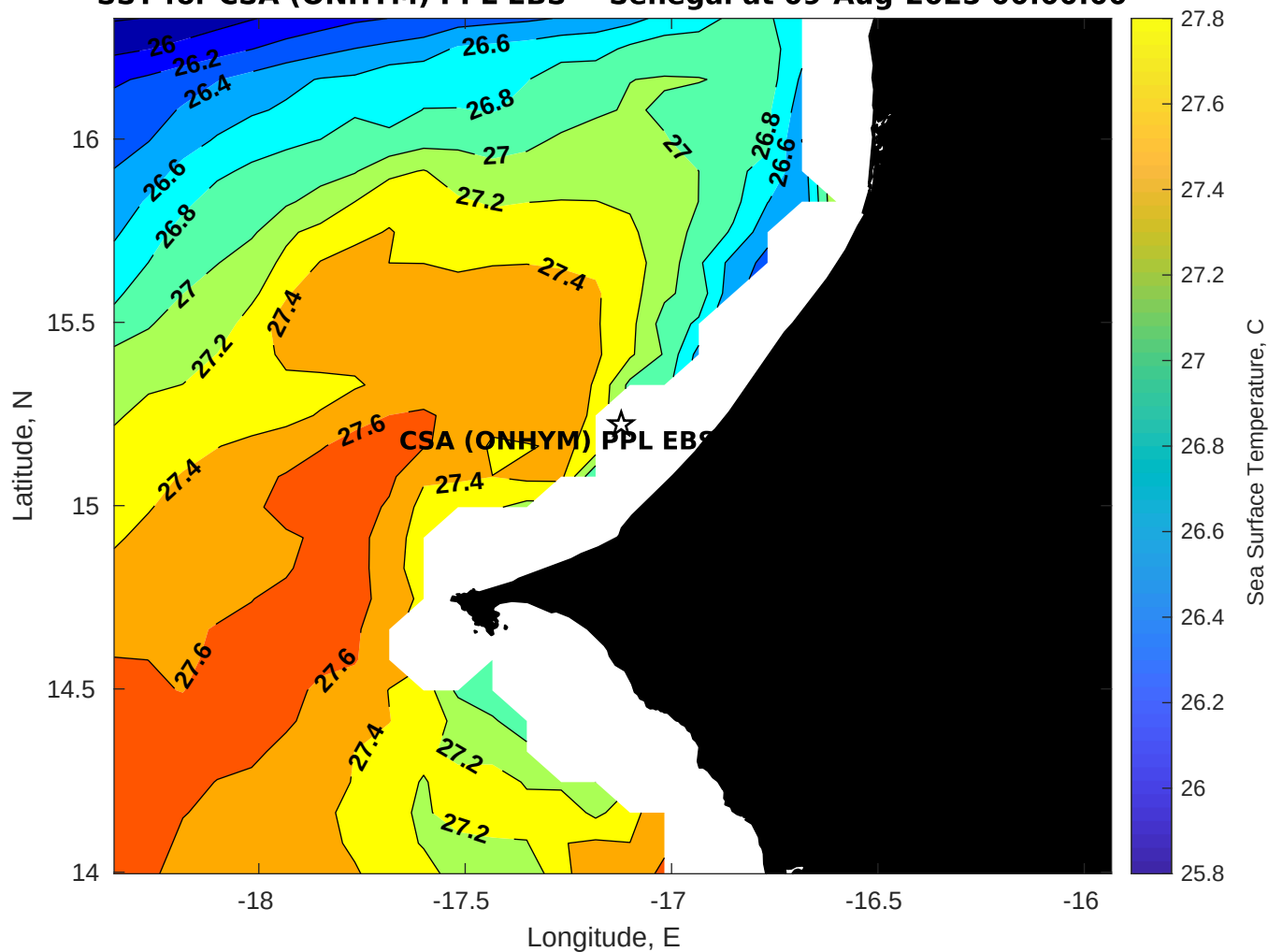
SST for CSA (ONHYM) PPL EBS - Senegal at 09-Aug-2025 00:00:00
