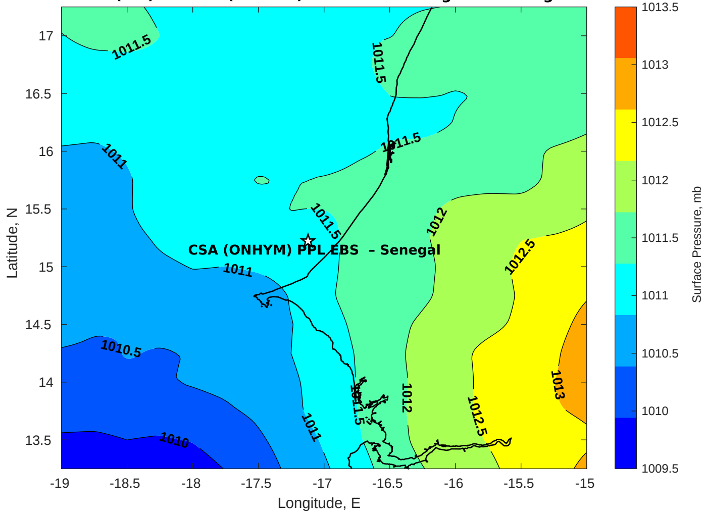
Surface Pressure (mb) for CSA (ONHYM) PPL EBS - Senegal at 10-Aug-2025 00:00:00
