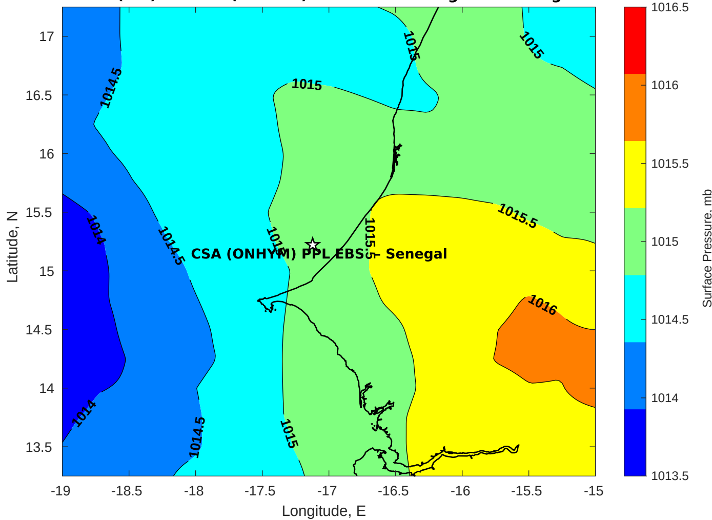
Surface Pressure (mb) for CSA (ONHYM) PPL EBS - Senegal at 11-Aug-2025 00:00:00
