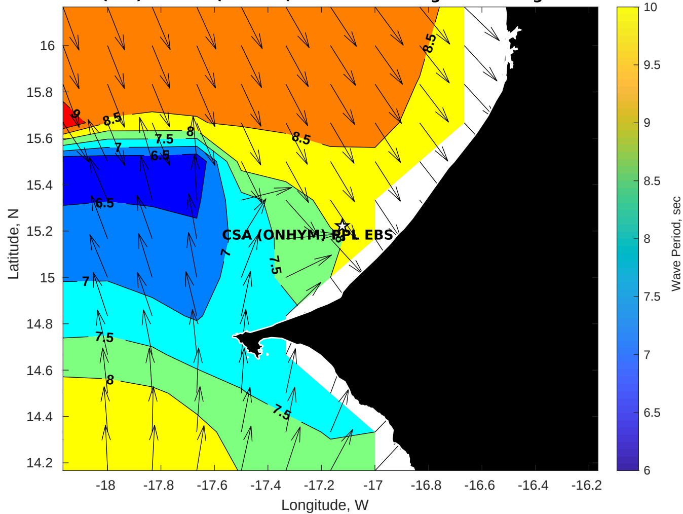
Wave Period (sec) for CSA (ONHYM) PPL EBS - Senegal at 10-Aug-2025 09:00:00
