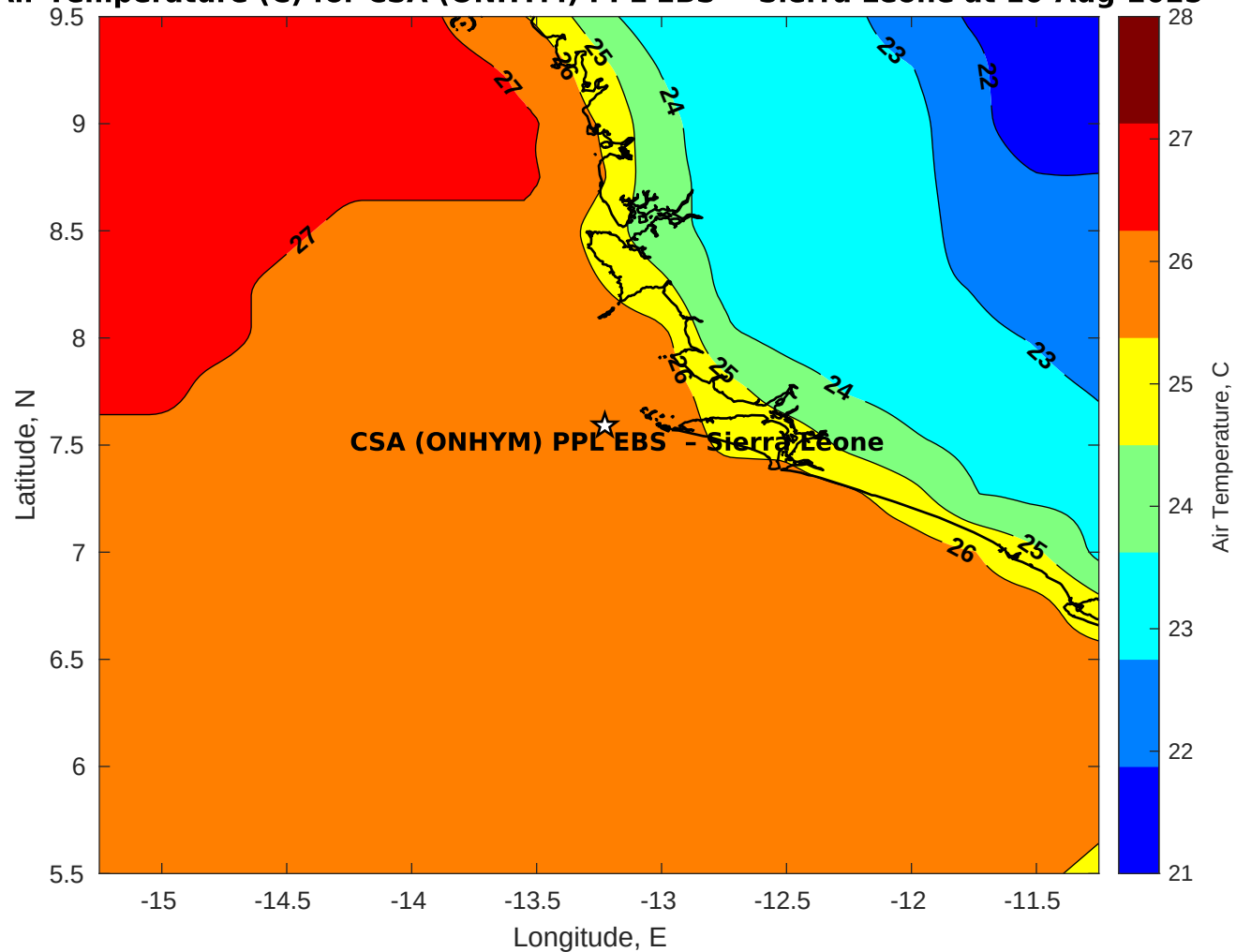
Air Temperature (C) for CSA (ONHYM) PPL EBS - Sierra Leone at 10-Aug-2025
