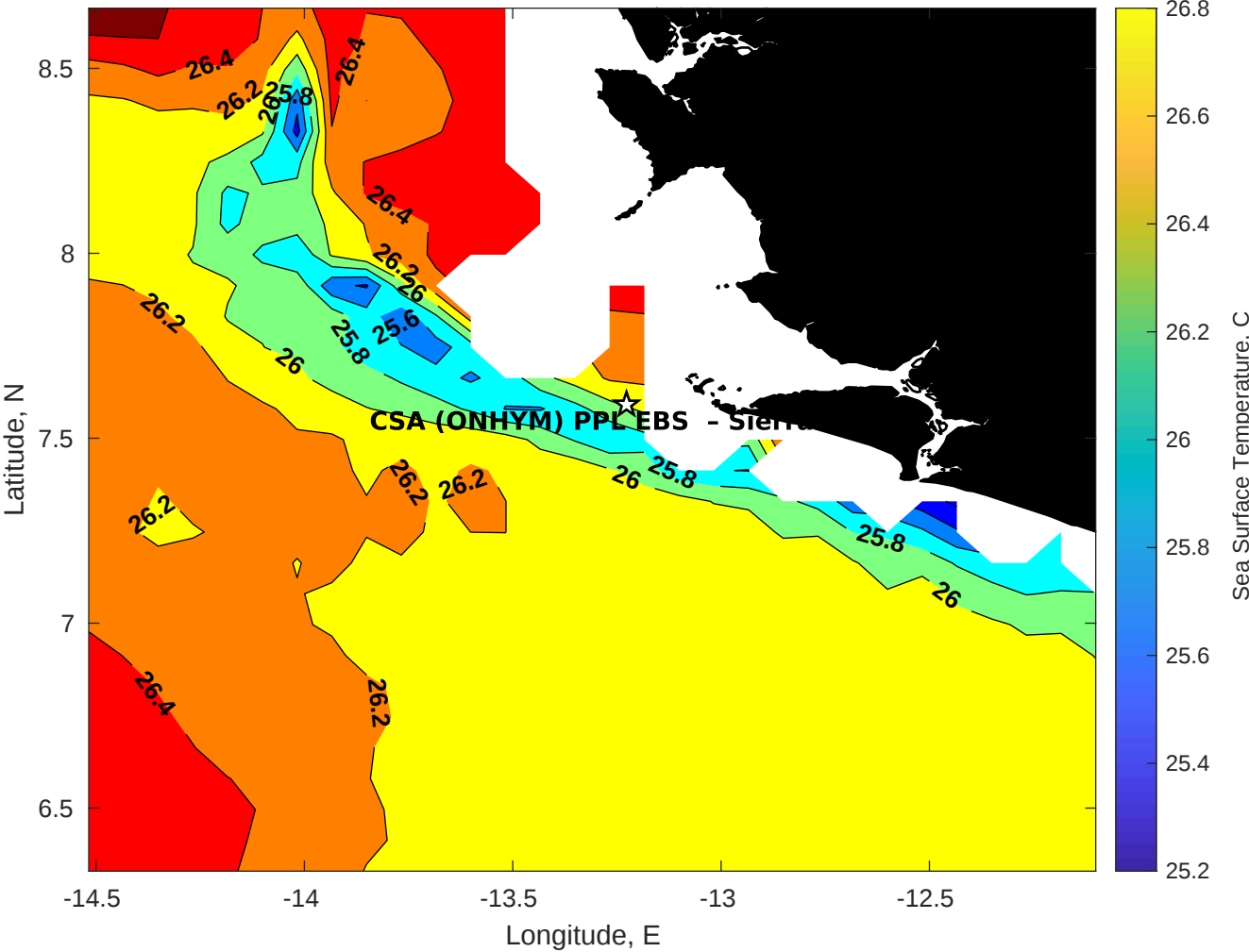
SST for CSA (ONHYM) PPL EBS - Sierra Leone at 09-Aug-2025 00:00:00
