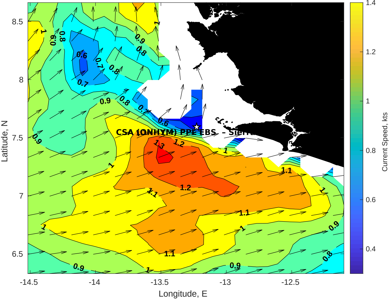
Surface Currents for CSA (ONHYM) PPL EBS - Sierra Leone at 09-Aug-2025 00:00:00
