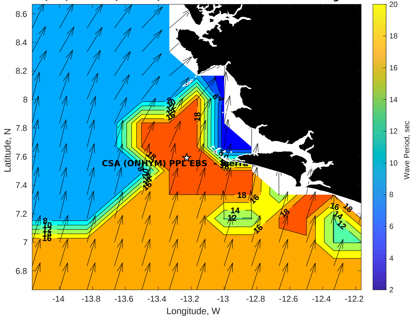
Wave Period (sec) for CSA (ONHYM) PPL EBS - Sierra Leone at 10-Aug-2025 09:00:00
