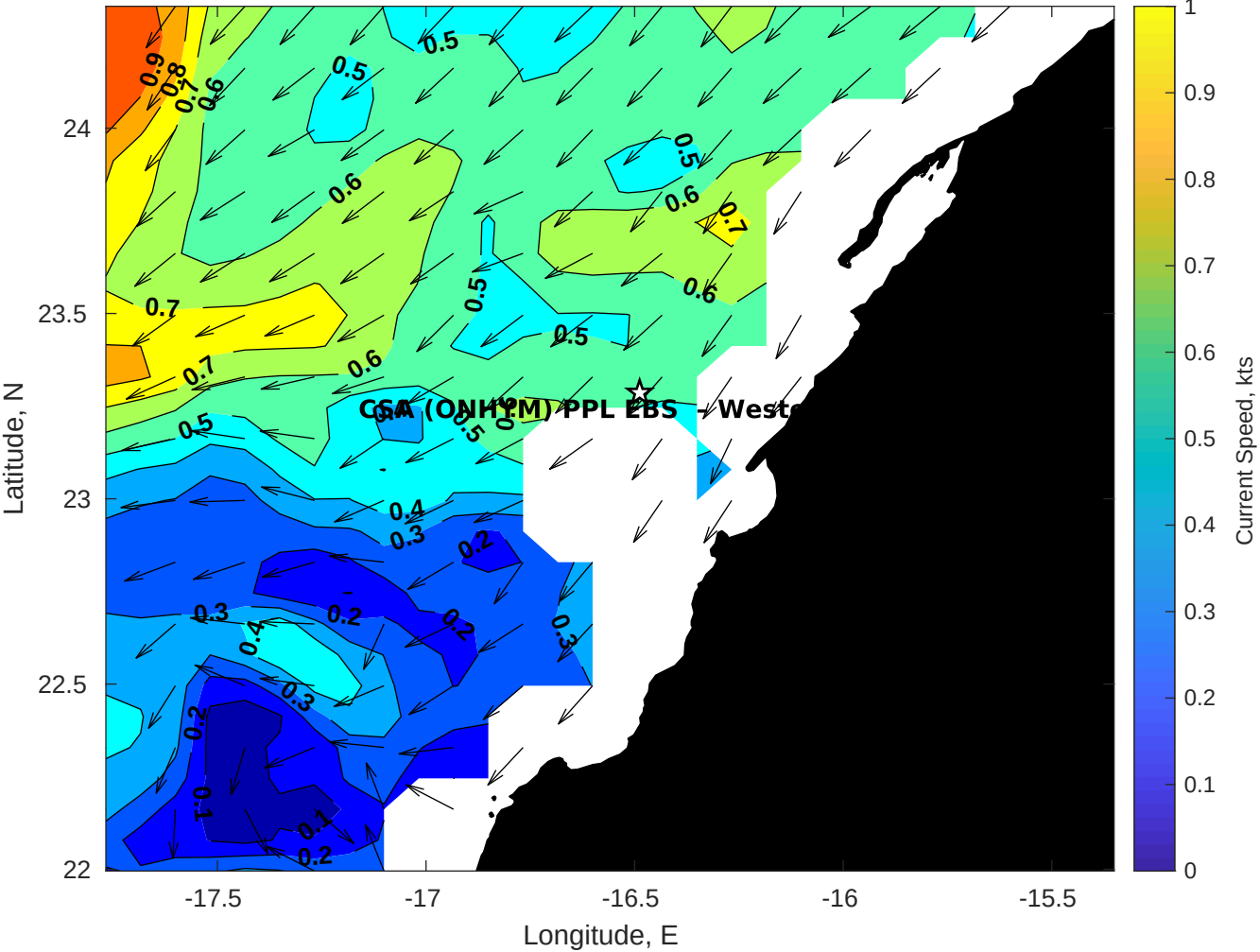
Surface Currents for CSA (ONHYM) PPL EBS - Western Sahara at 09-Aug-2025 00:00:00
