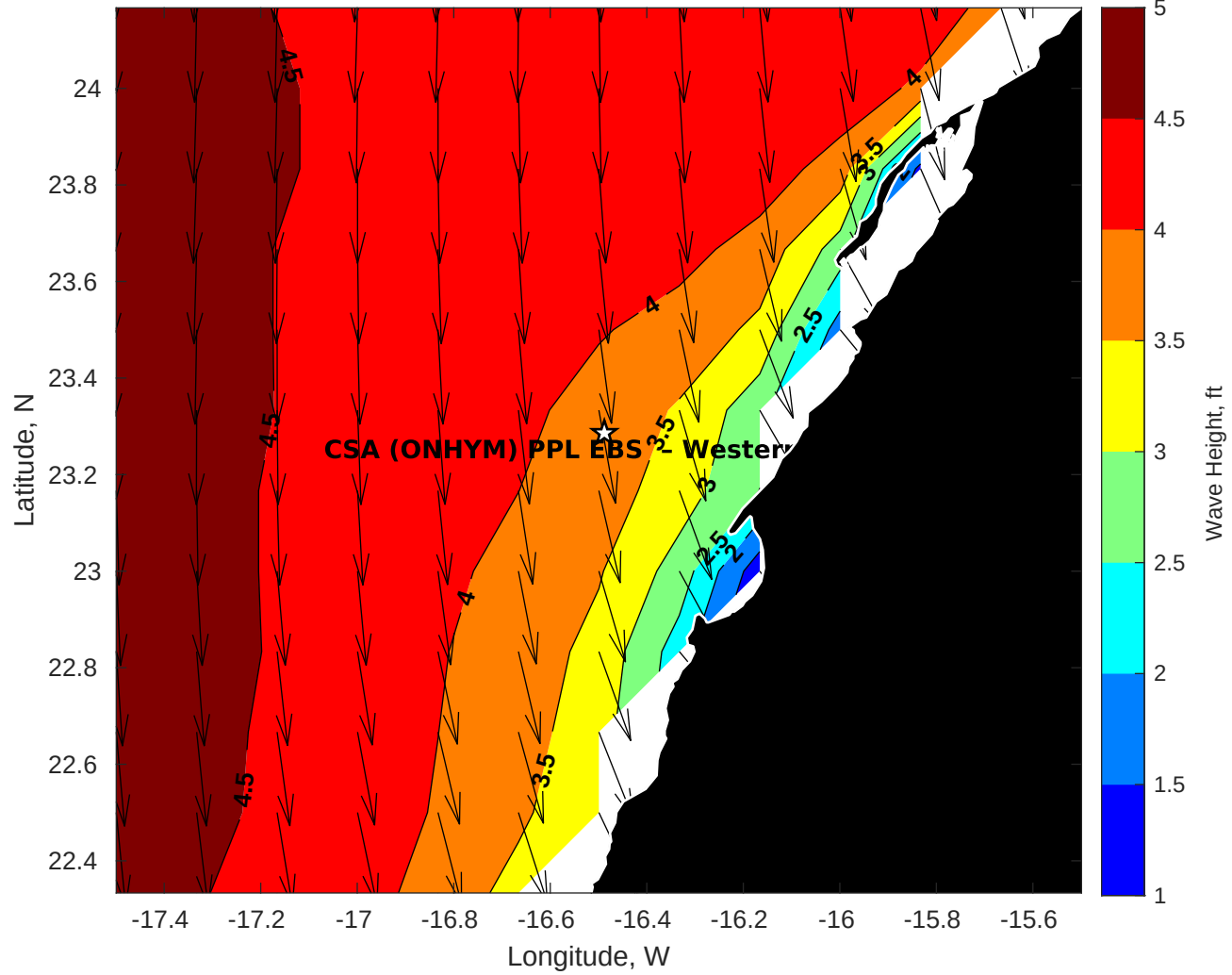
Wave Height (ft) for CSA (ONHYM) PPL EBS - Western Sahara at 10-Aug-2025 09:00:00
