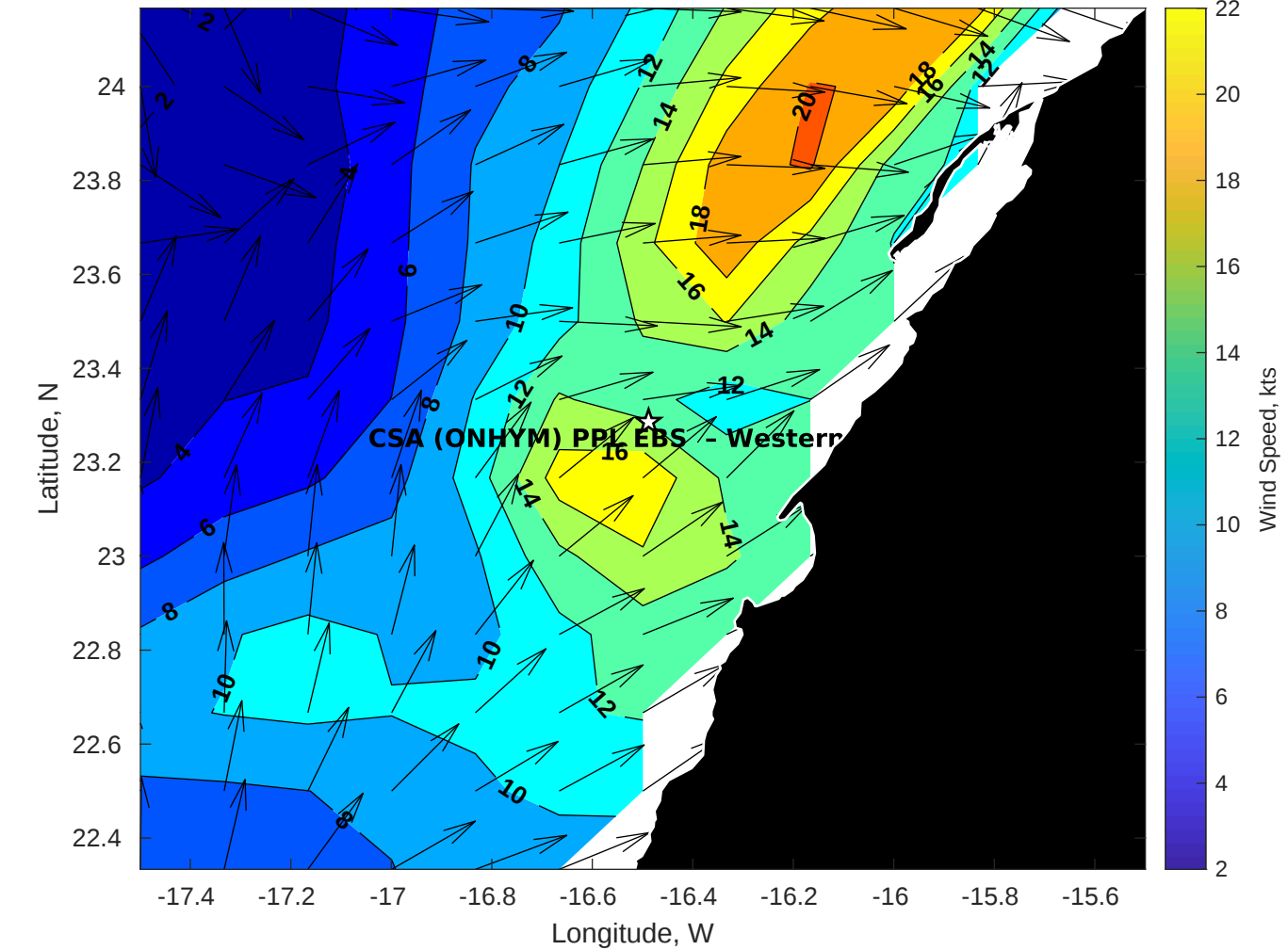
Winds (kts) for CSA (ONHYM) PPL EBS - Western Sahara at 10-Aug-2025 09:00:00
