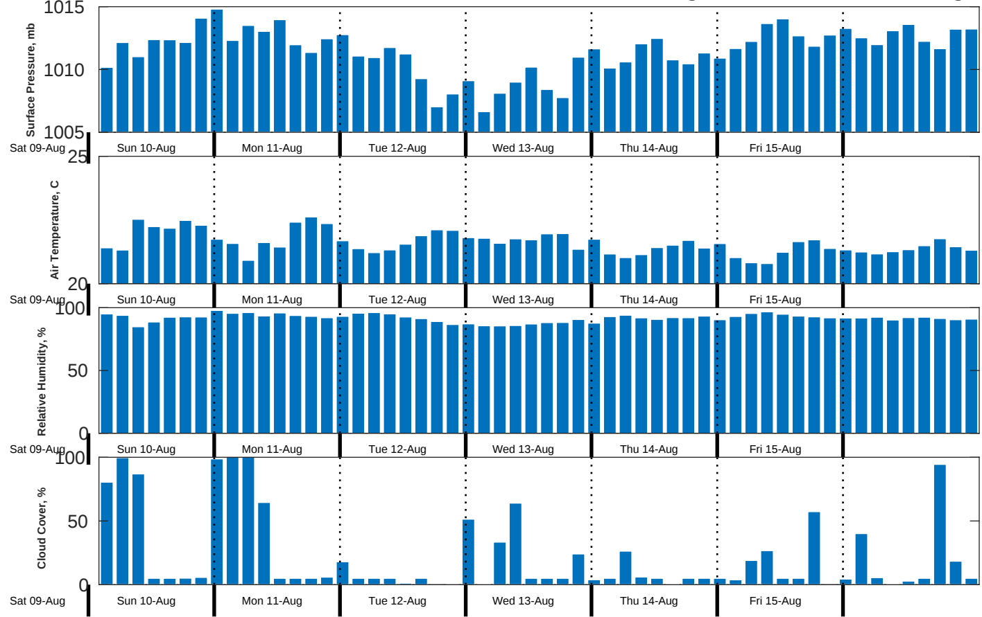
Met Forecast for CSA (ONHYM) PPL EBS - Western Sahara from 10-Aug-2025 00:00:00 to 17-Aug-2025 00:00:00
