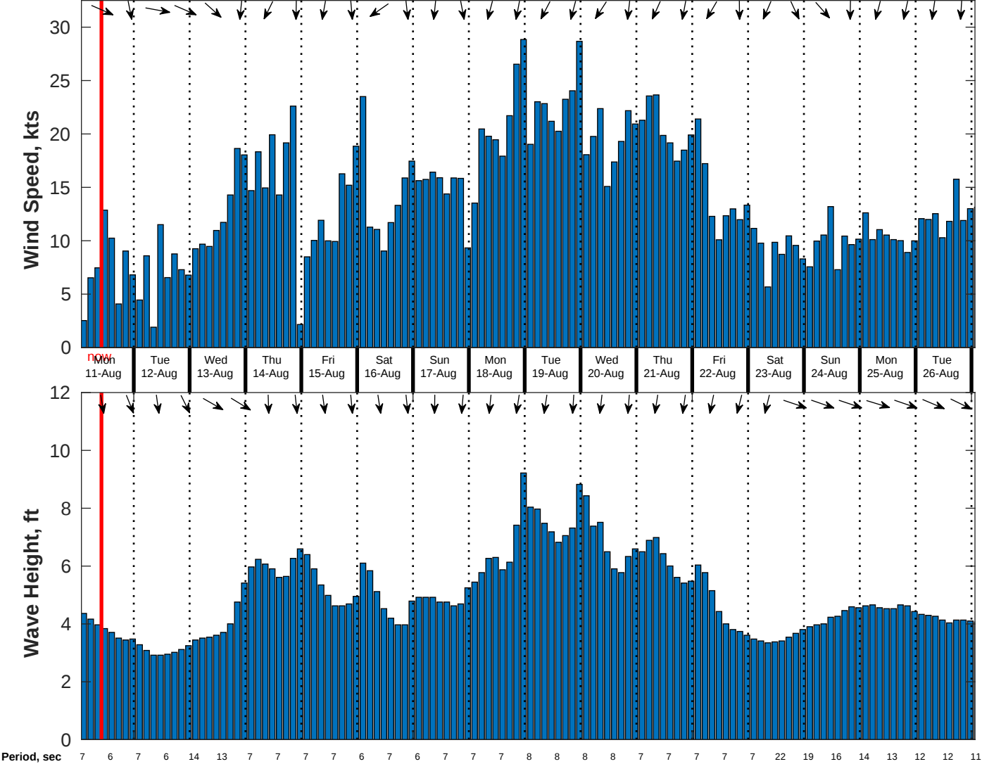
Wind & Wave Forecast for CSA (ONHYM) PPL EBS - Western Sahara from 10-Aug-2025 01:00:00 to 26-Aug-2025 01:00:00
