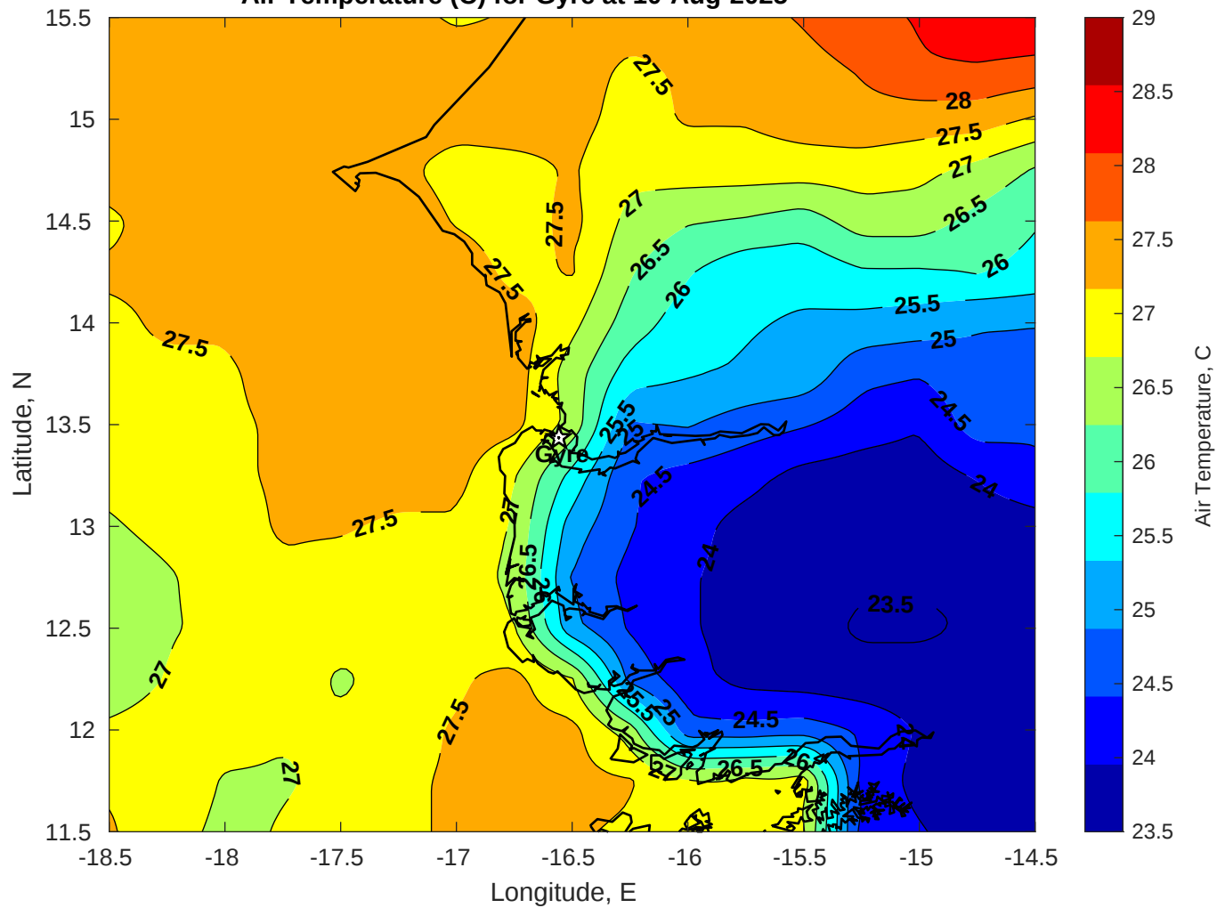
Air Temperature (C) for Gyre at 10-Aug-2025
