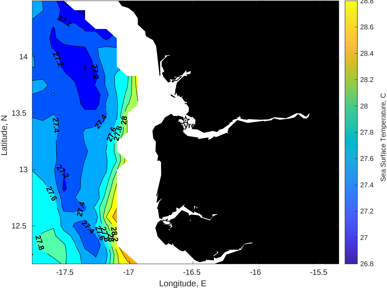
SST for Gyre at 09-Aug-2025 00:00:00
