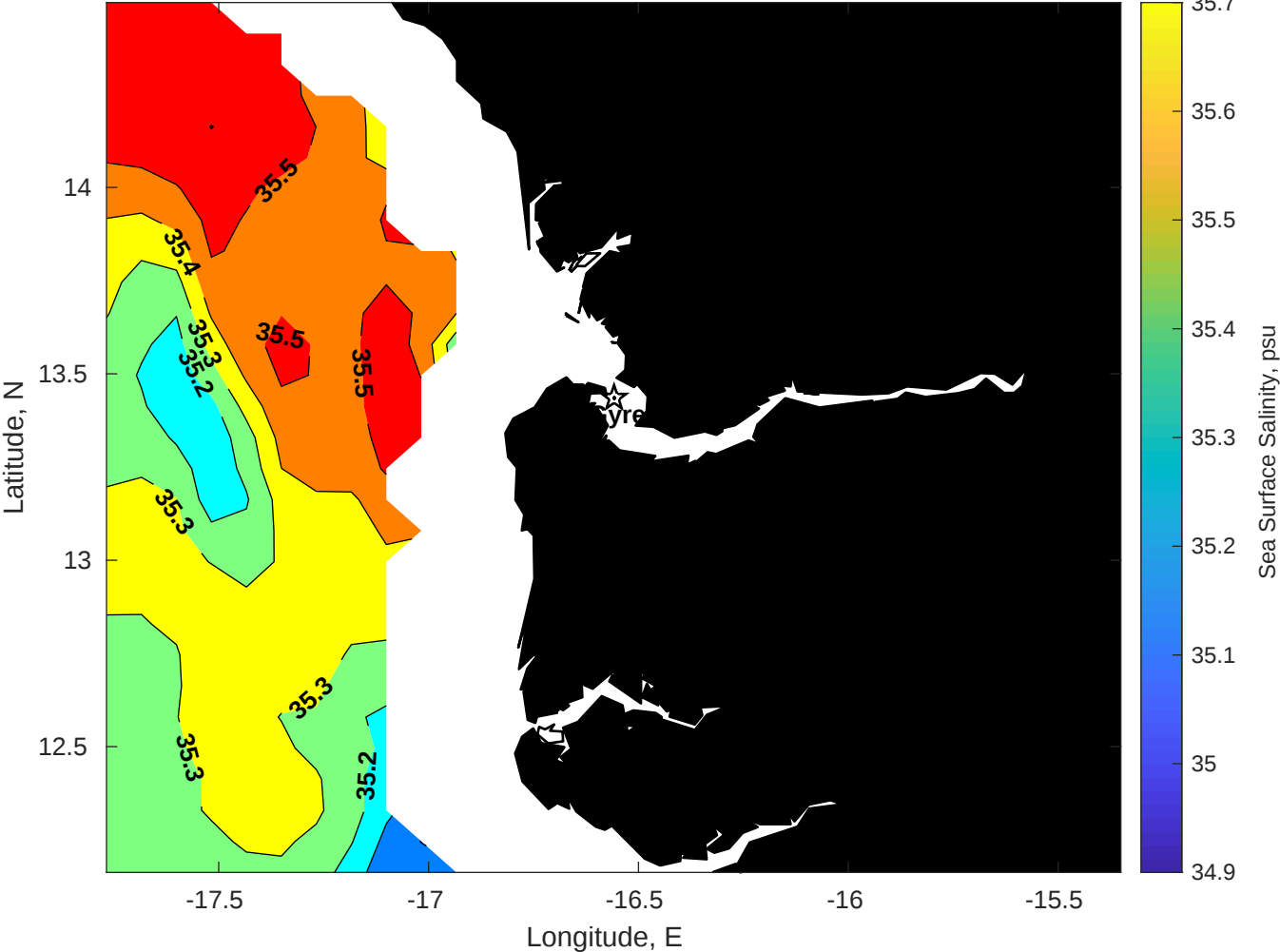
Surface Salinity for Gyre at 09-Aug-2025 00:00:00
