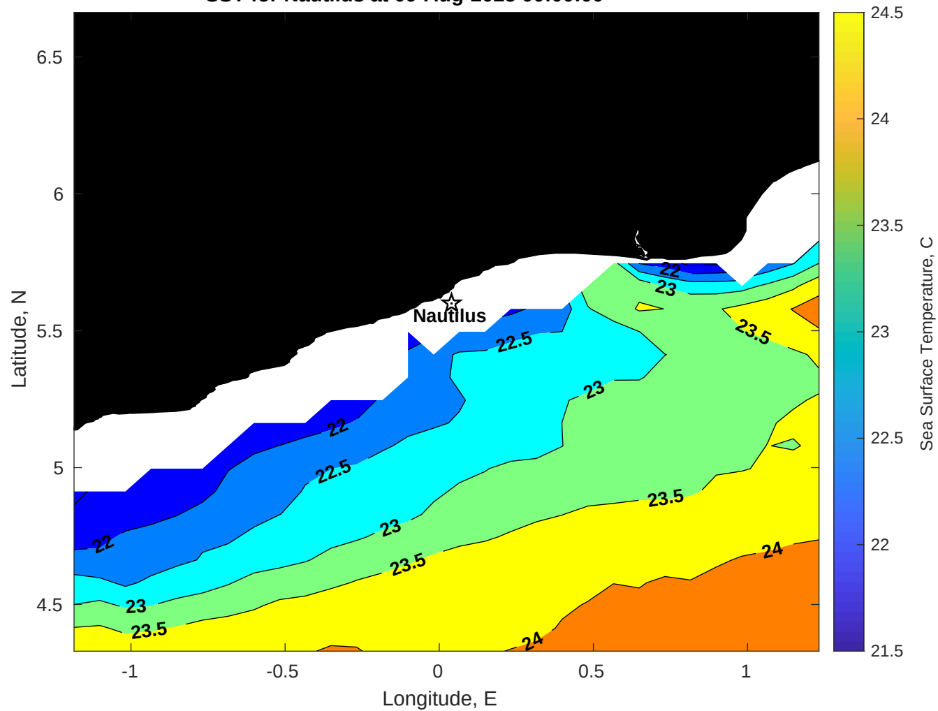
SST for Nautilus at 09-Aug-2025 00:00:00
