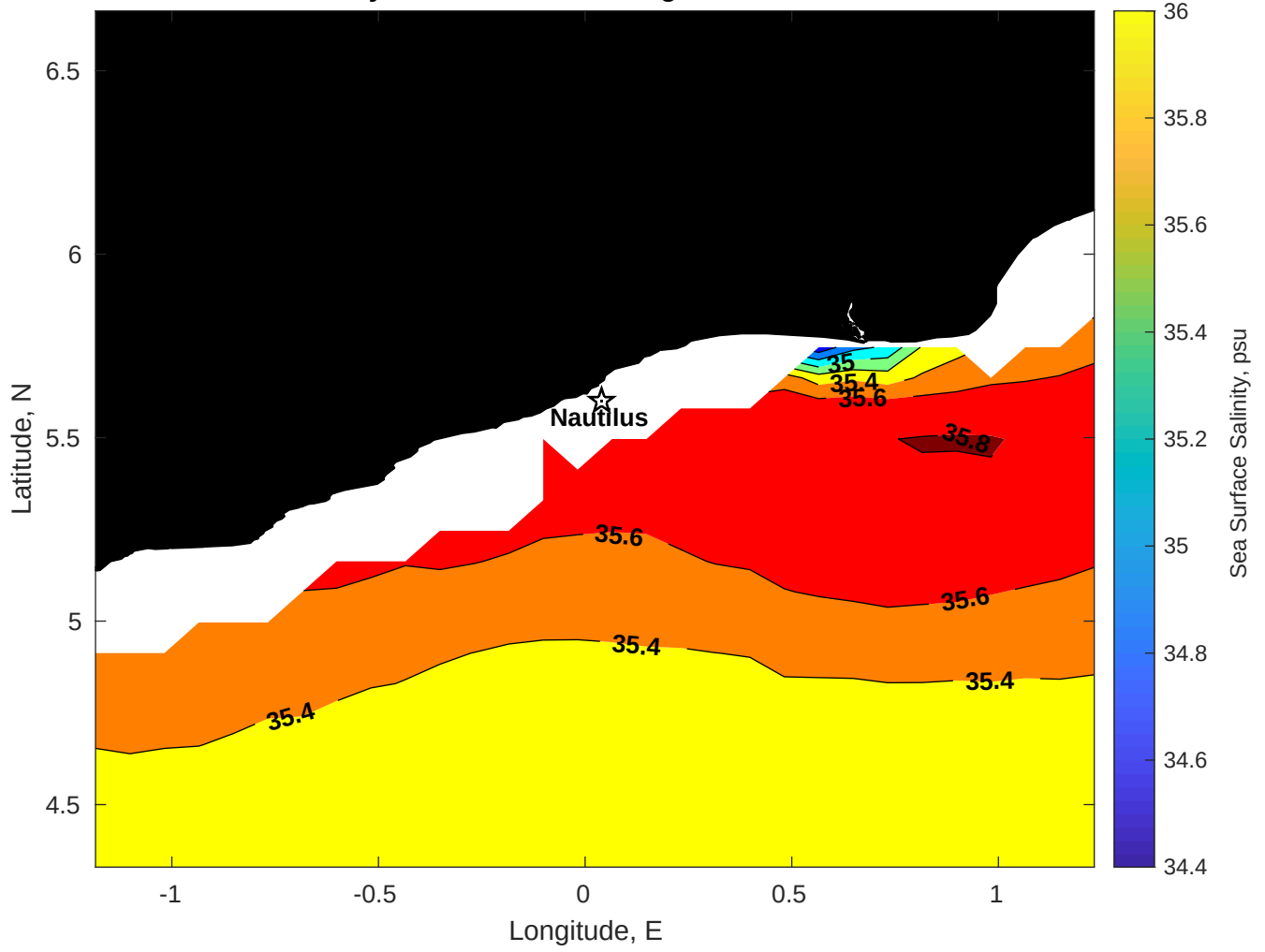
Surface Salinity for Nautilus at 09-Aug-2025 00:00:00
