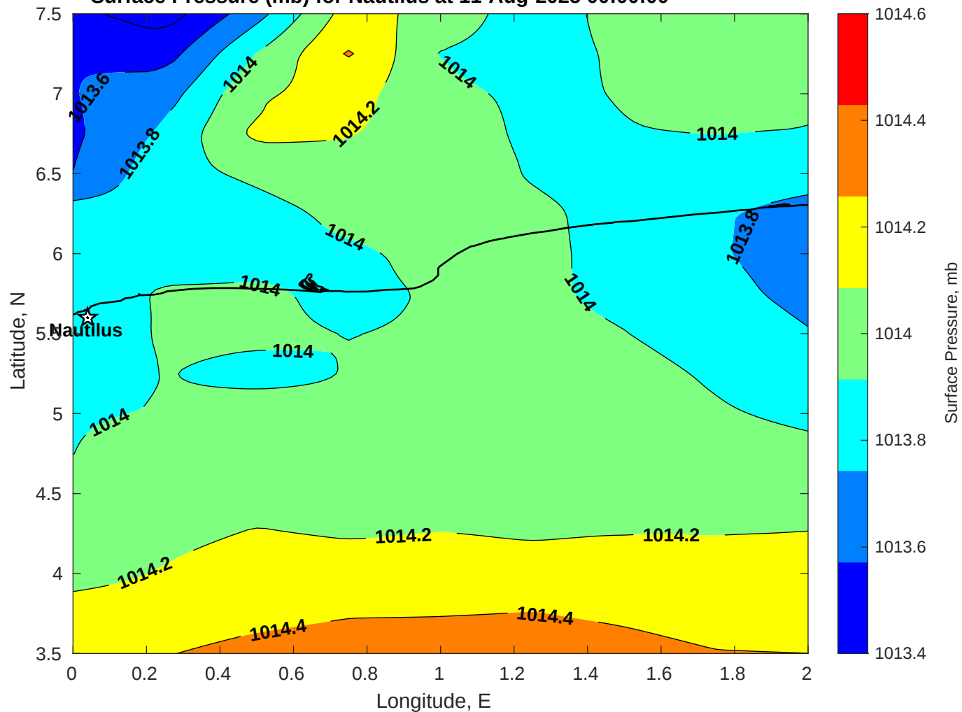
Surface Pressure (mb) for Nautilus at 11-Aug-2025 00:00:00
