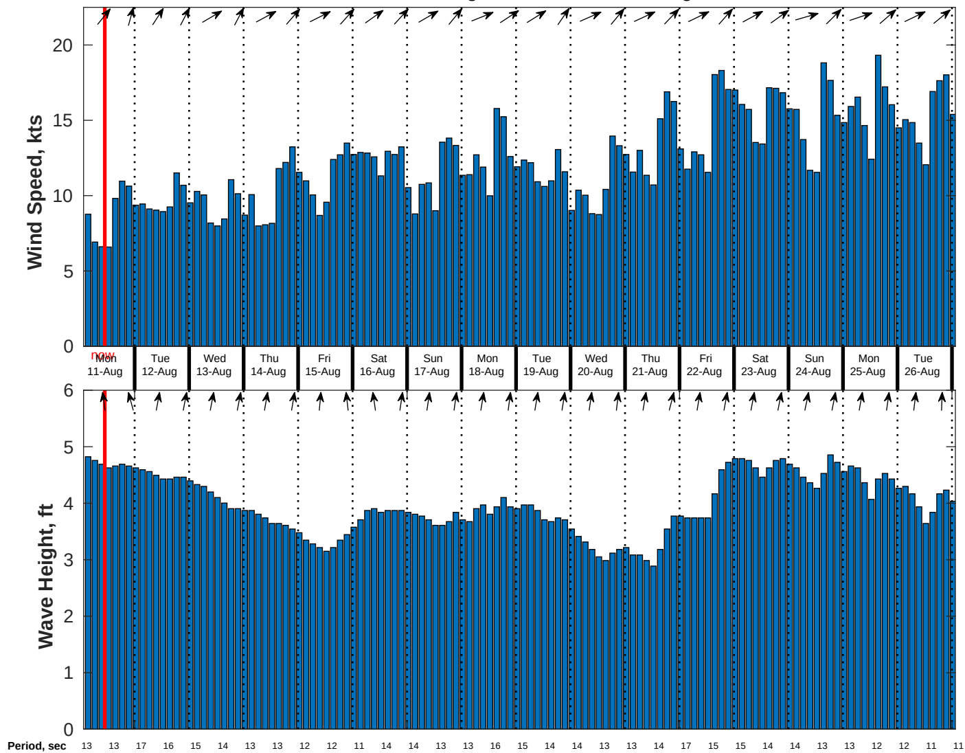
Wind & Wave Forecast for Nautilus from 10-Aug-2025 02:00:00 to 26-Aug-2025 02:00:00
