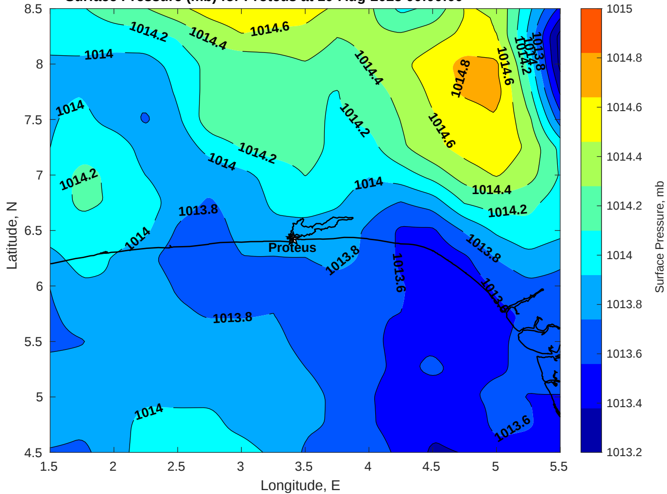
Surface Pressure (mb) for Proteus at 10-Aug-2025 00:00:00
