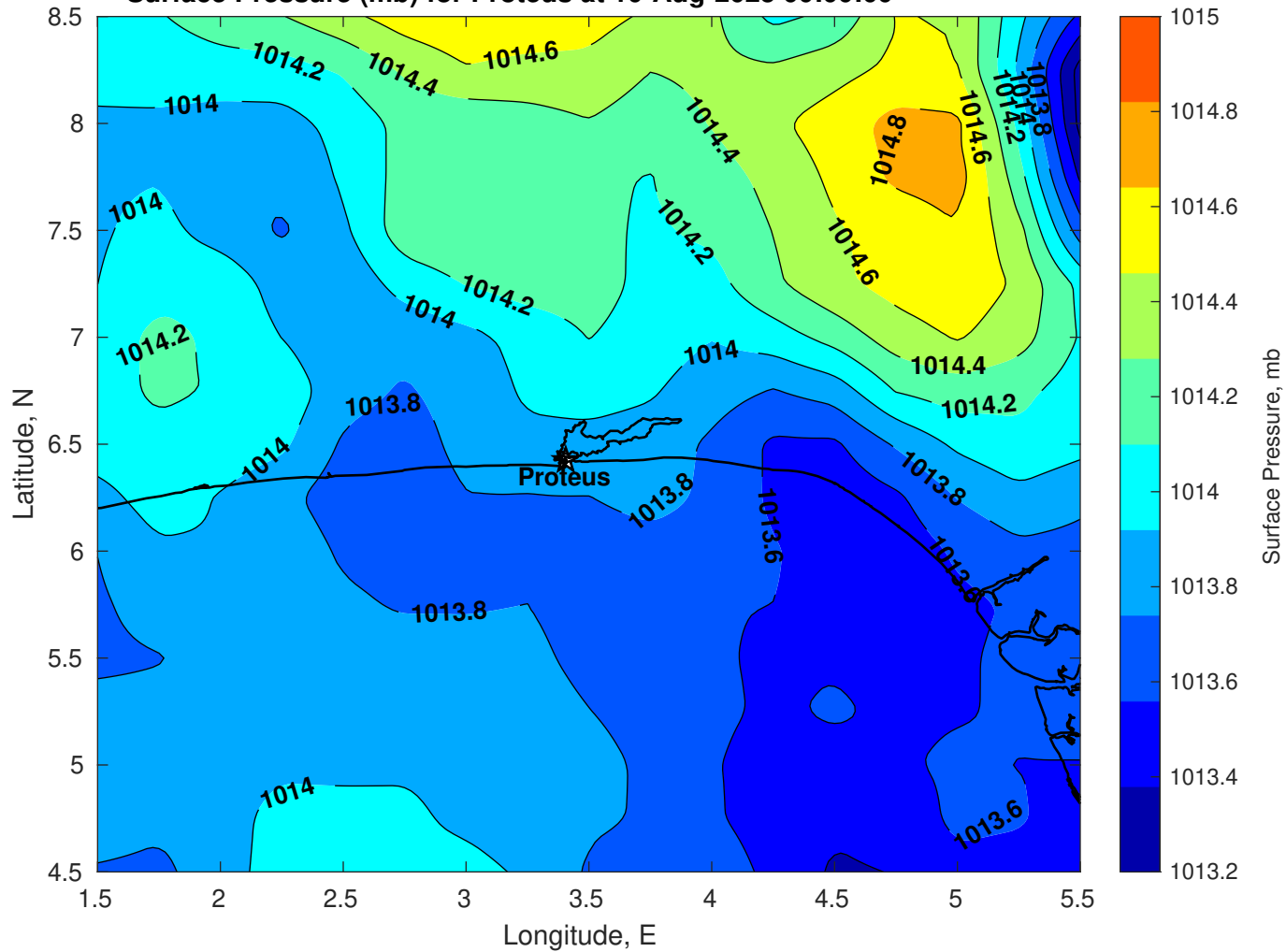
Surface Pressure (mb) for Proteus at 10-Aug-2025 00:00:00
