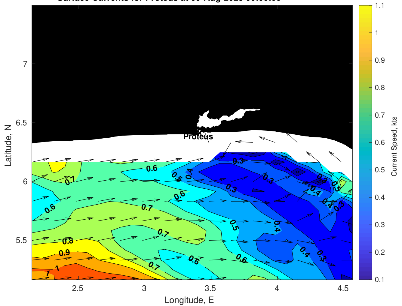
Surface Currents for Proteus at 09-Aug-2025 00:00:00
