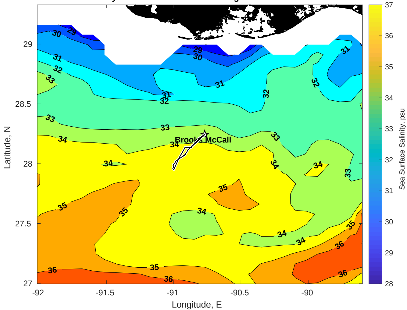
Surface Salinity for Brooks McCall at 10-Aug-2025 00:00:00
