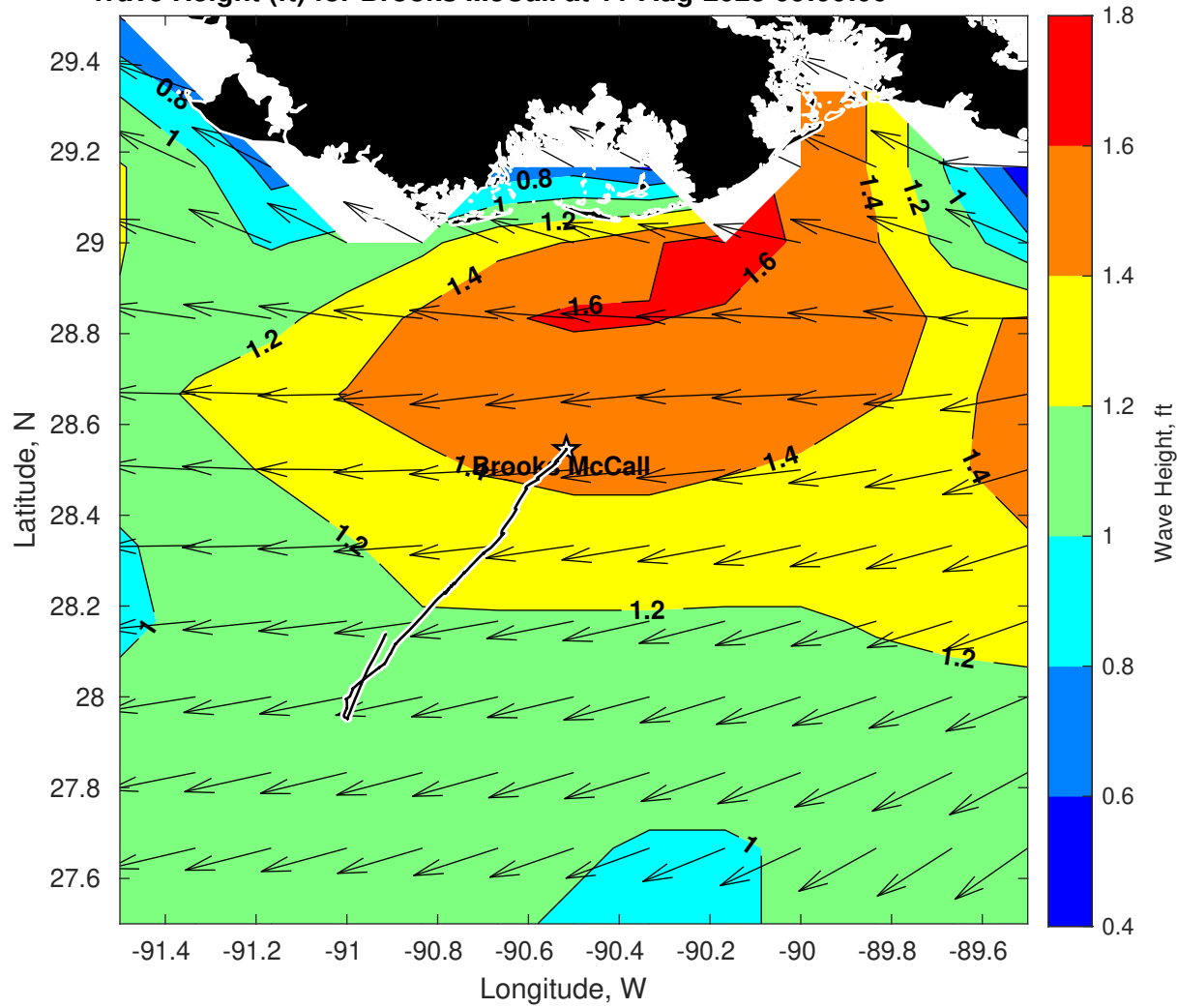
Wave Height (ft) for Brooks McCall at 11-Aug-2025 09:00:00
