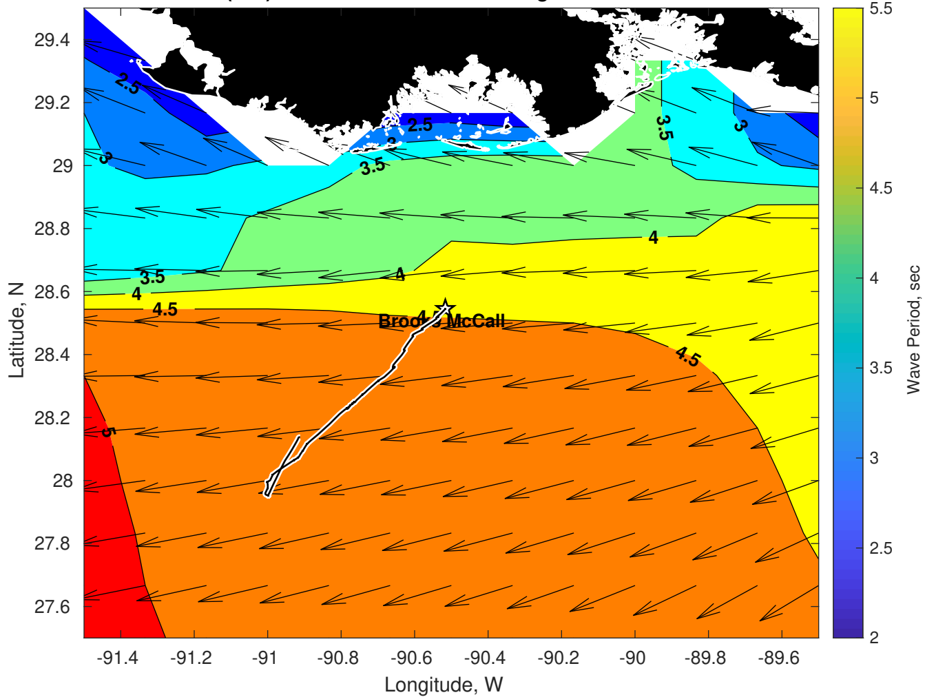
Wave Period (sec) for Brooks McCall at 11-Aug-2025 09:00:00
