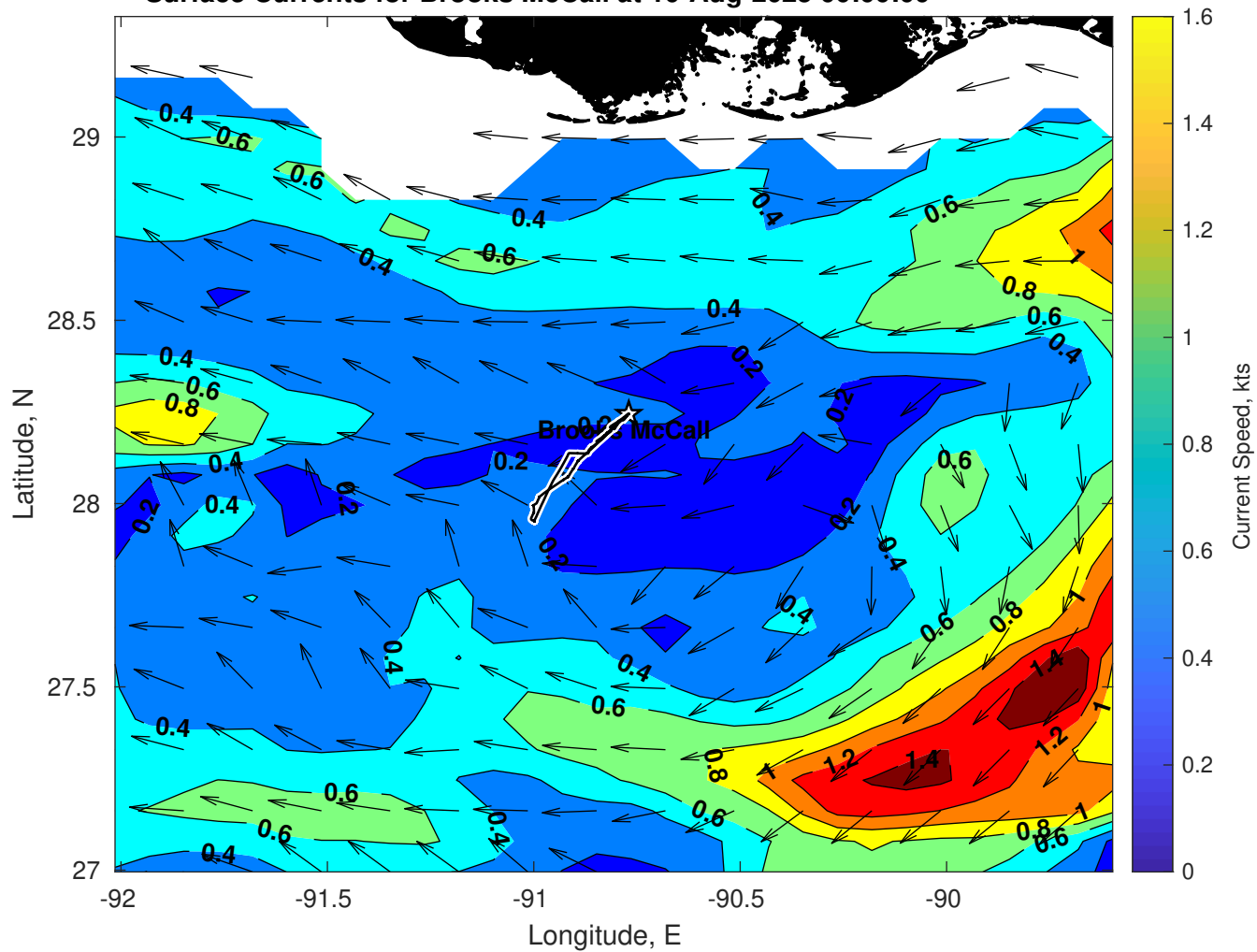
Surface Currents for Brooks McCall at 10-Aug-2025 00:00:00
