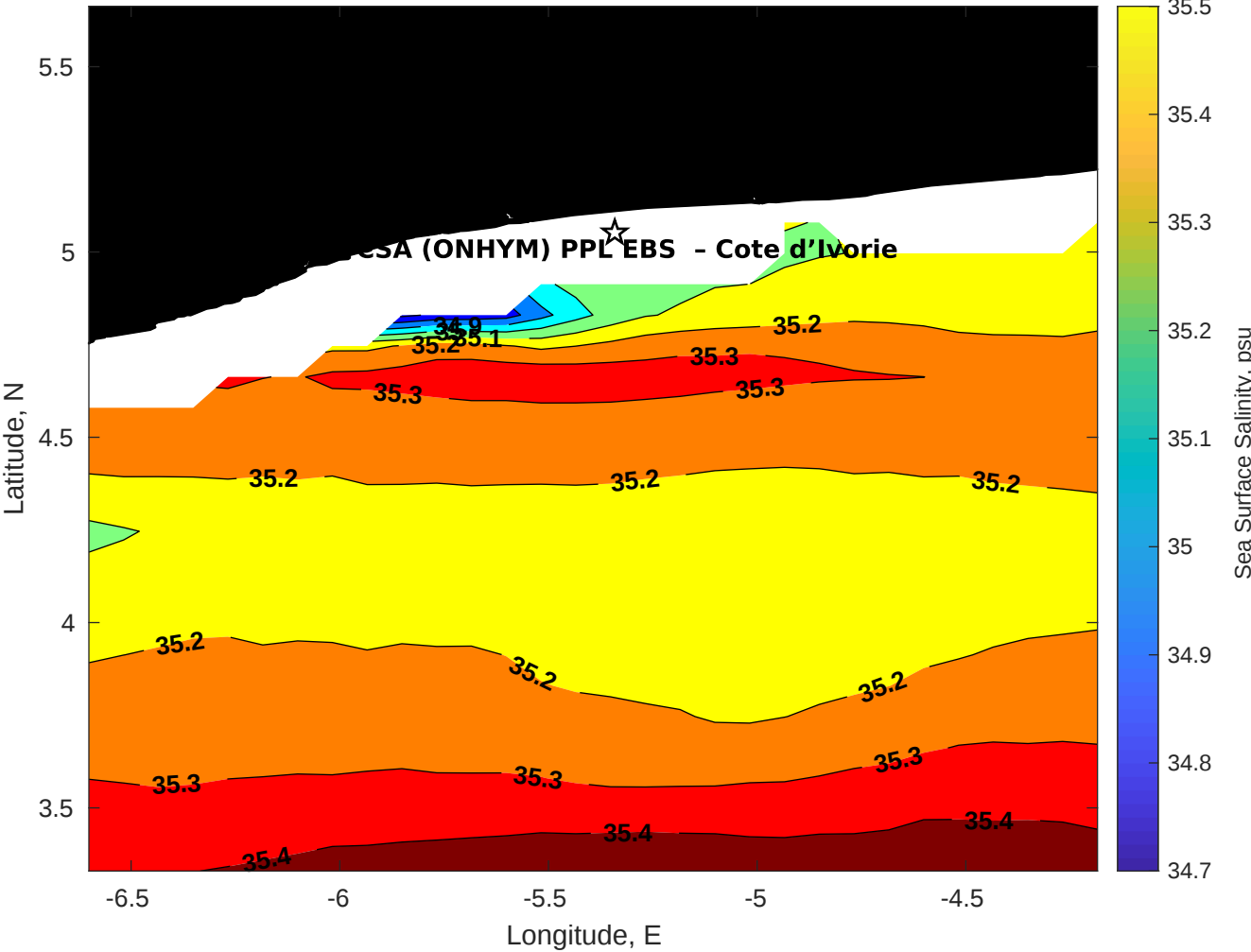
Surface Salinity for CSA (ONHYM) PPL EBS - Cote d'Ivoire at 10-Aug-2025 00:00:00
