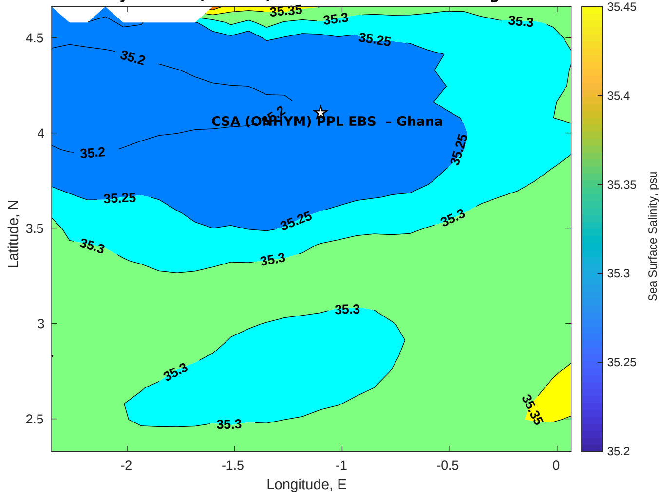
Surface Salinity for CSA (ONHYM) PPL EBS - Ghana at 10-Aug-2025 00:00:00
