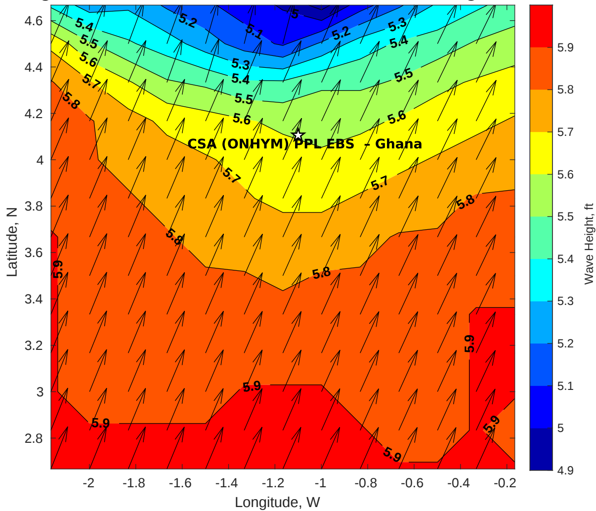
Wave Height (ft) for CSA (ONHYM) PPL EBS - Ghana at 11-Aug-2025 09:00:00
