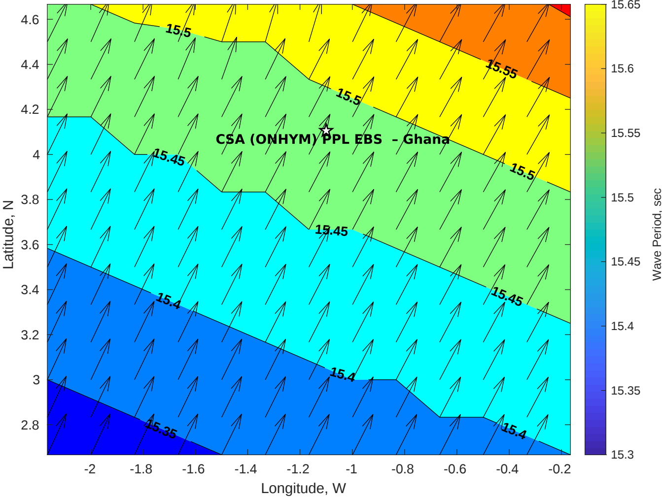
Wave Period (sec) for CSA (ONHYM) PPL EBS - Ghana at 11-Aug-2025 09:00:00
