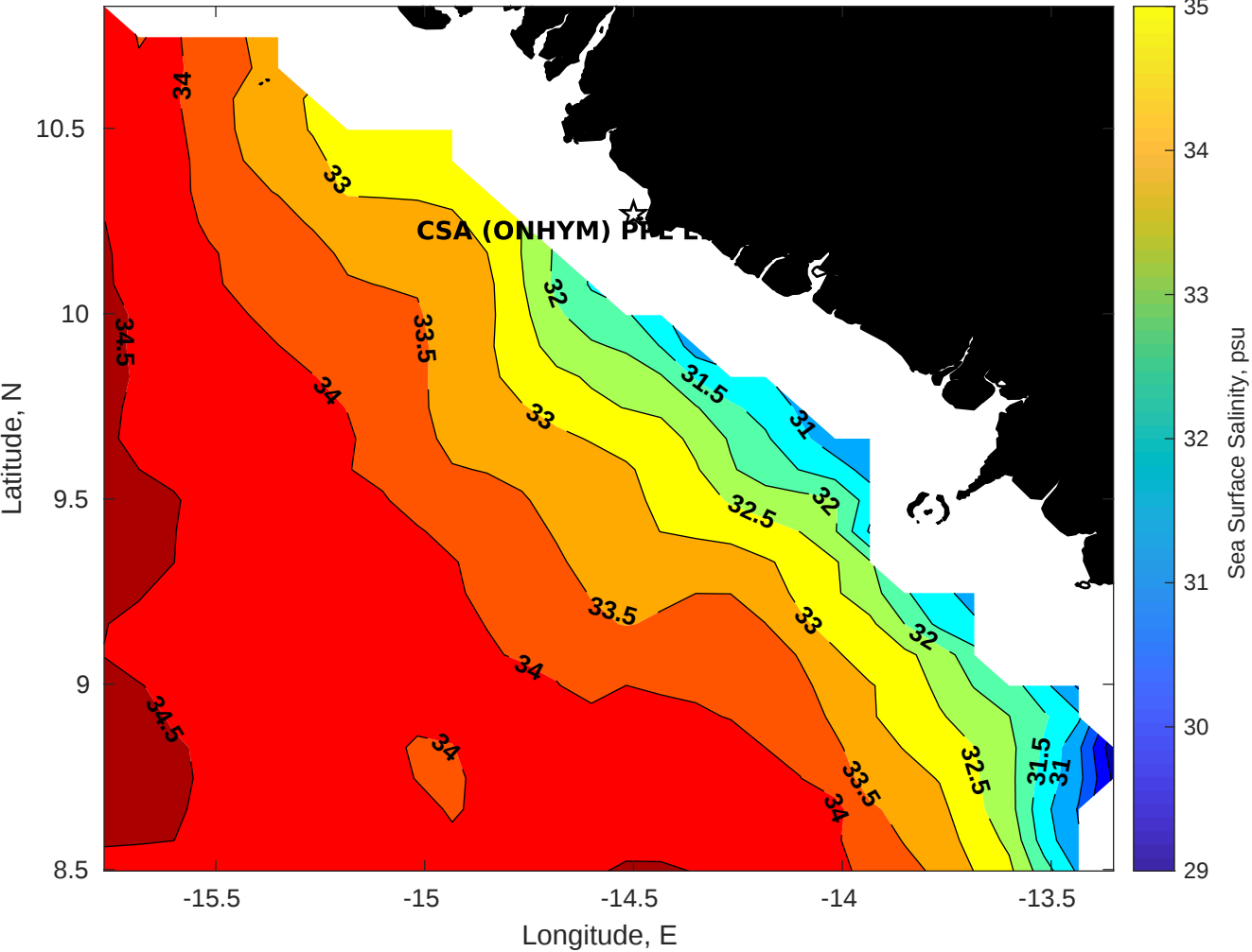
Surface Salinity for CSA (ONHYM) PPL EBS - Guinea at 10-Aug-2025 00:00:00
