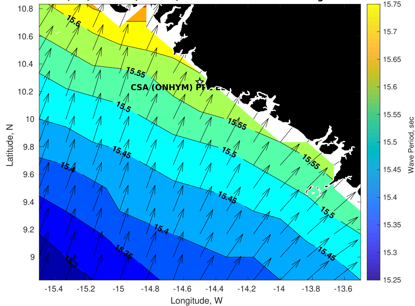
Wave Period (sec) for CSA (ONHYM) PPL EBS - Guinea at 11-Aug-2025 09:00:00
