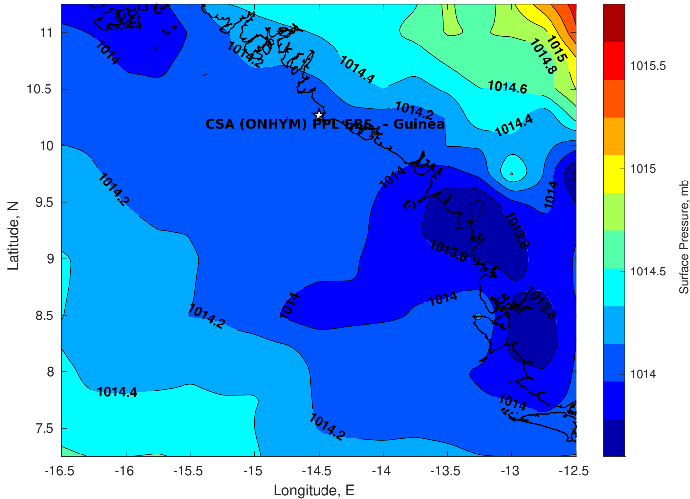
Surface Pressure (mb) for CSA (ONHYM) PPL EBS - Guinea at 12-Aug-2025 00:00:00
