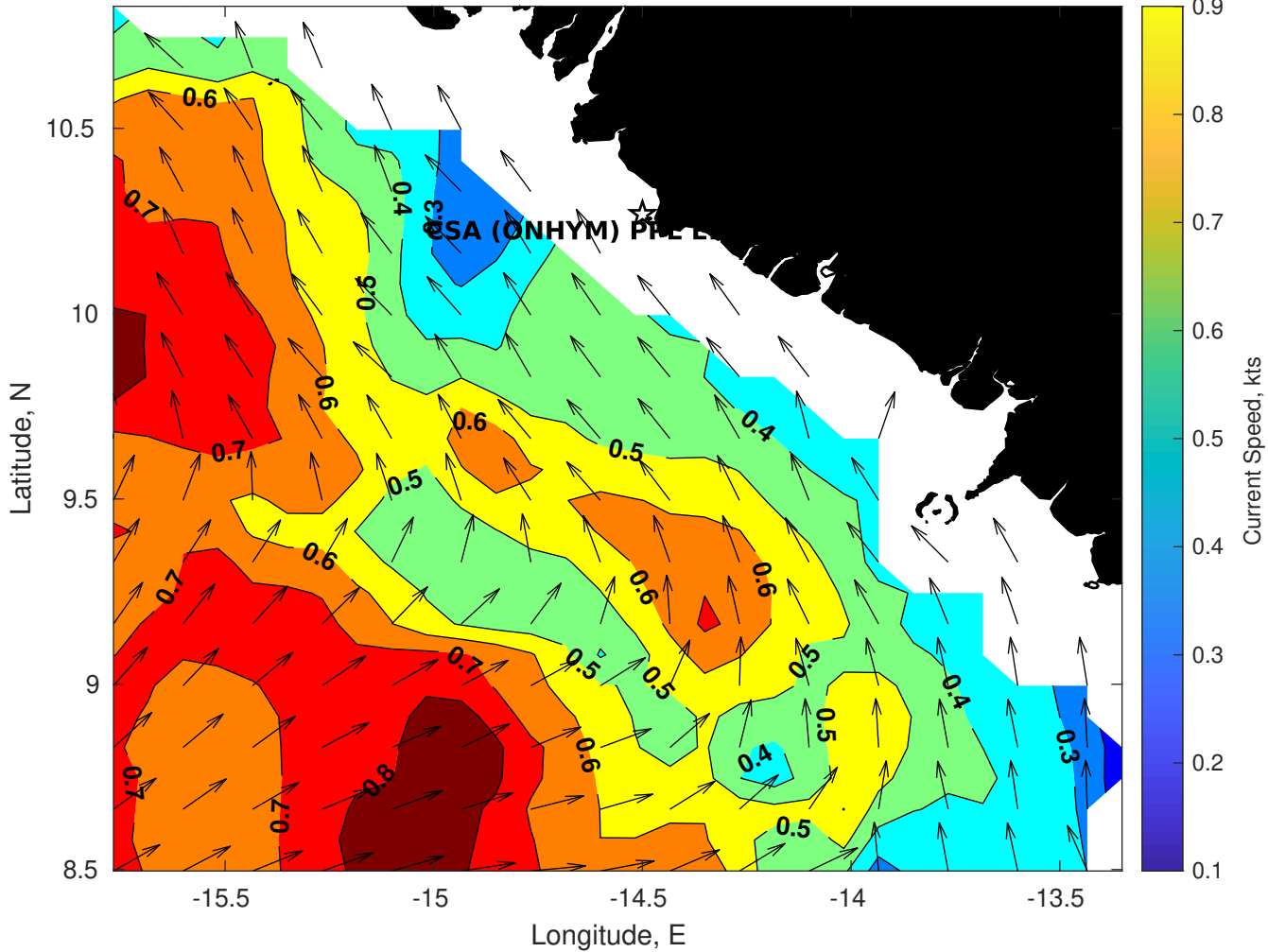
Surface Currents for CSA (ONHYM) PPL EBS - Guinea at 10-Aug-2025 00:00:00
