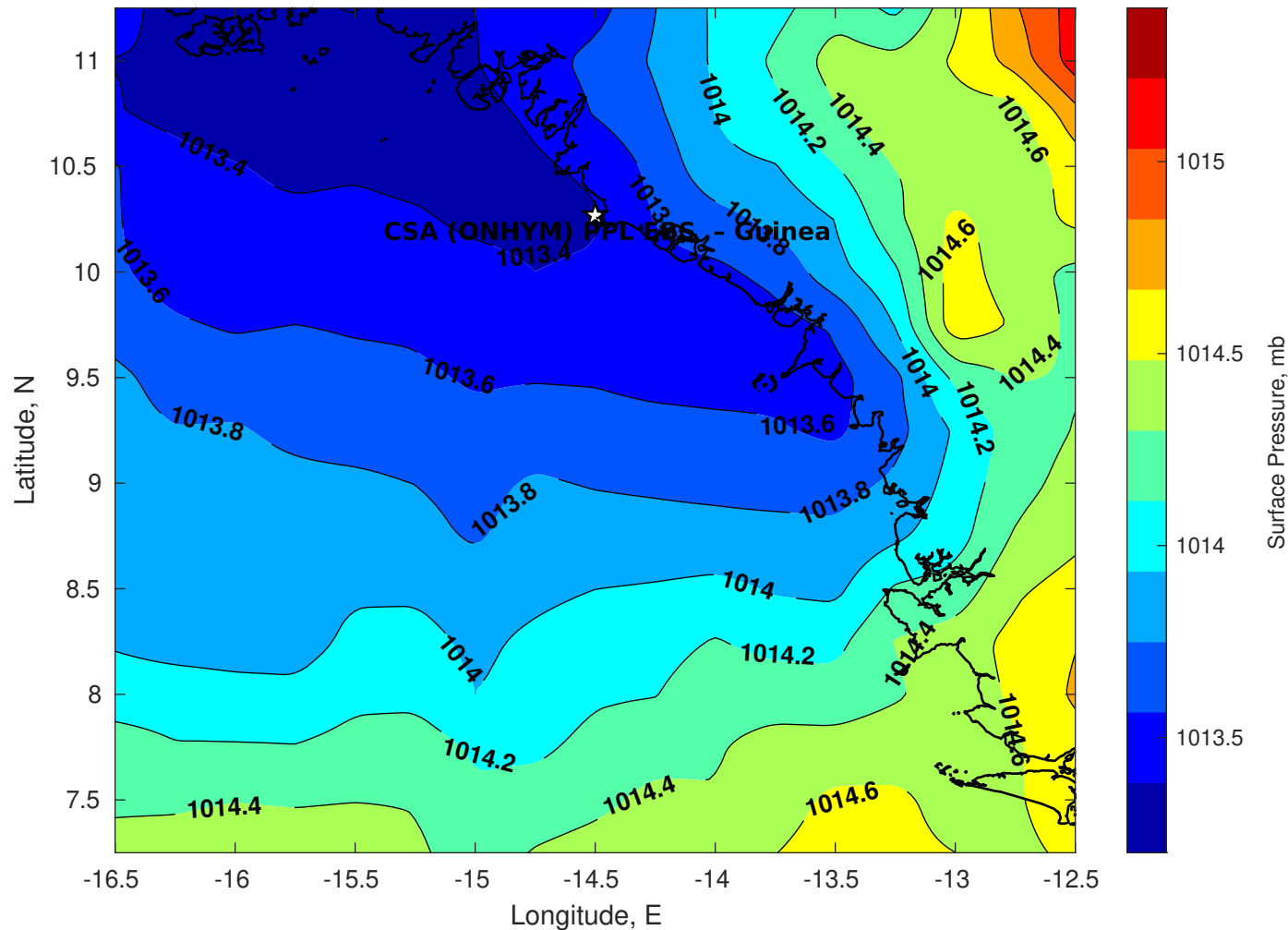
Surface Pressure (mb) for CSA (ONHYM) PPL EBS - Guinea at 13-Aug-2025 00:00:00
