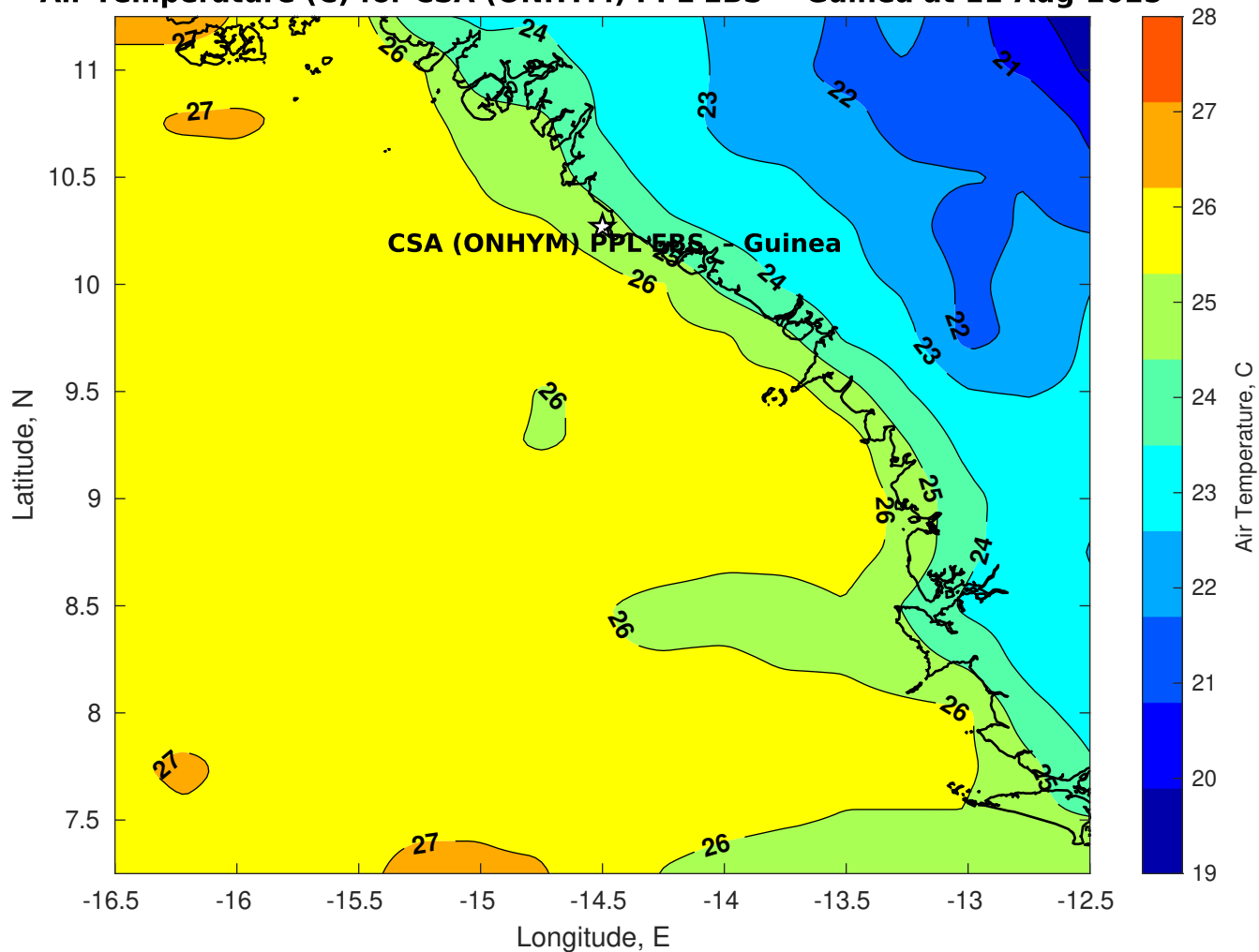
Air Temperature (C) for CSA (ONHYM) PPL EBS - Guinea at 11-Aug-2025
