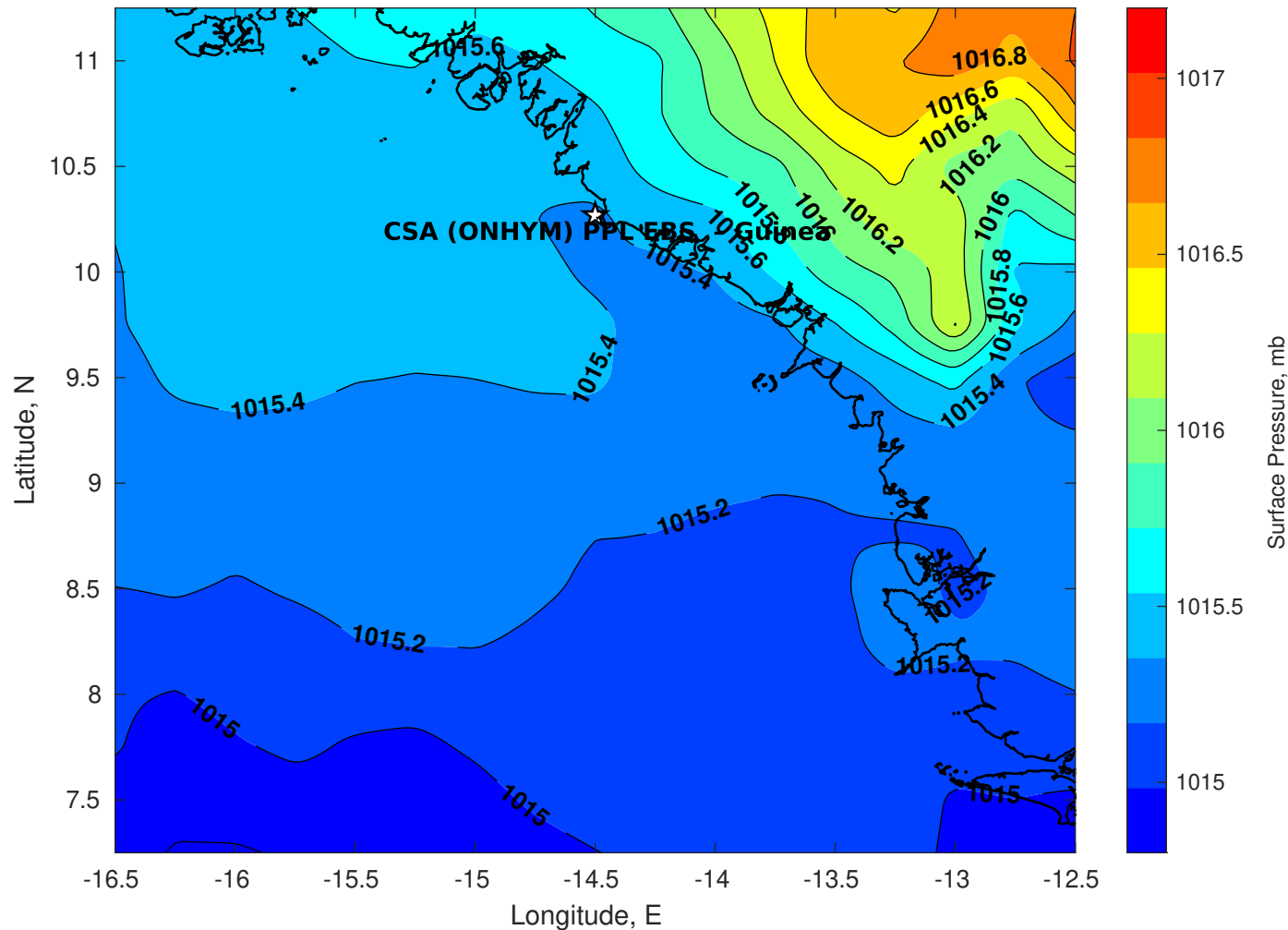
Surface Pressure (mb) for CSA (ONHYM) PPL EBS - Guinea at 11-Aug-2025 00:00:00
