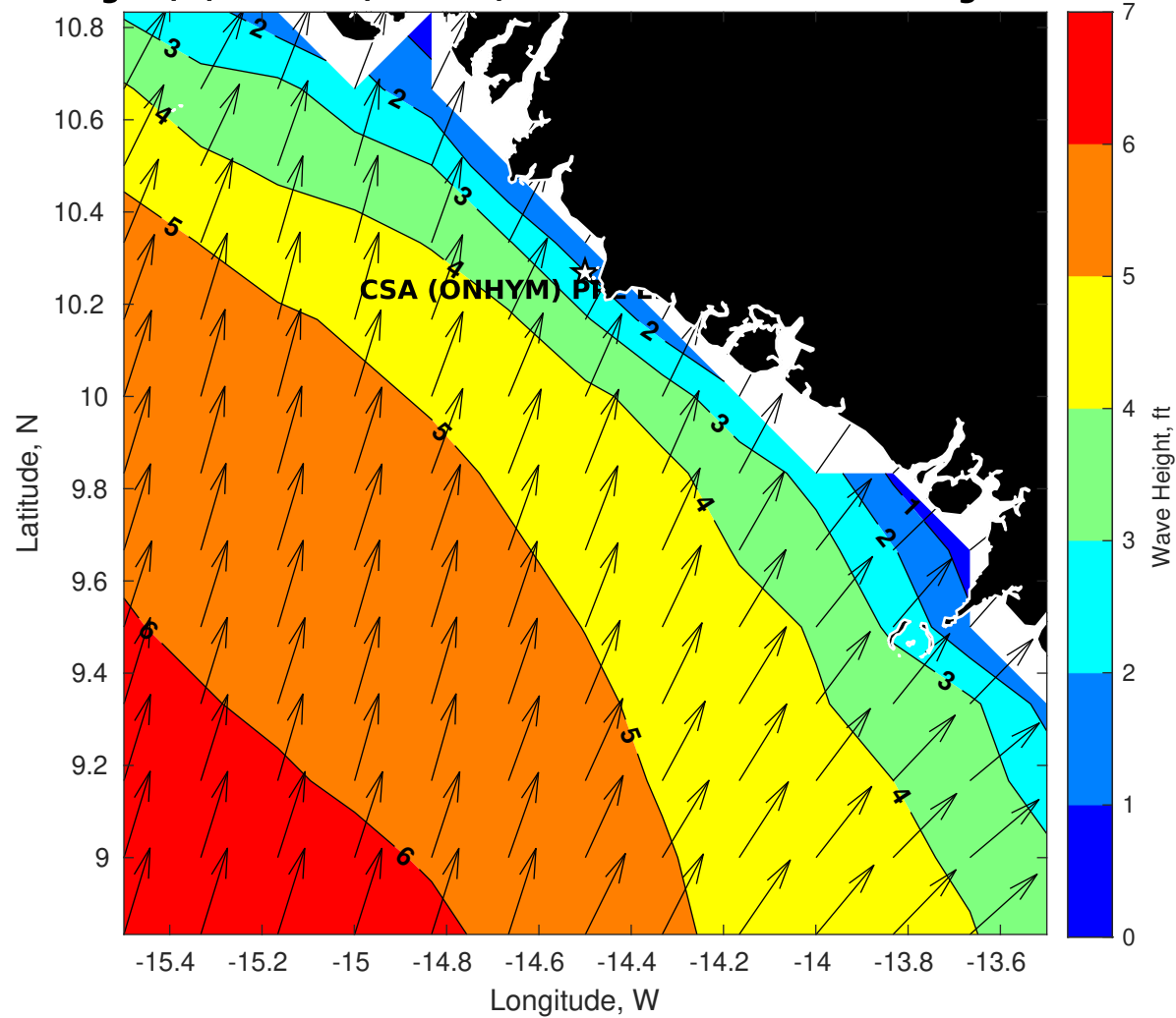
Wave Height (ft) for CSA (ONHYM) PPL EBS - Guinea at 11-Aug-2025 09:00:00
