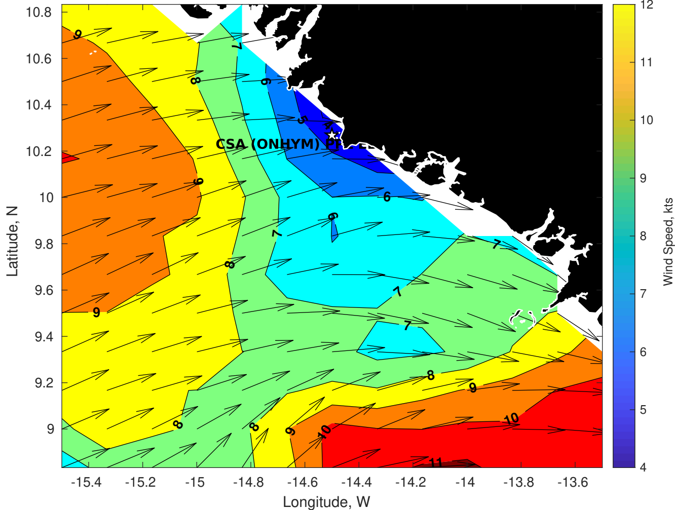
Winds (kts) for CSA (ONHYM) PPL EBS - Guinea at 11-Aug-2025 09:00:00
