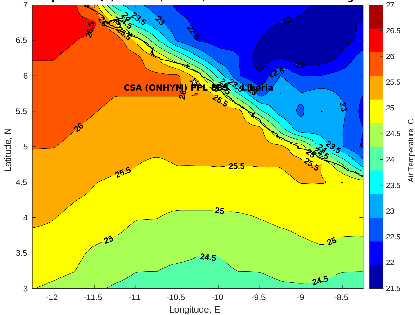
Air Temperature (C) for CSA (ONHYM) PPL EBS - Liberia at 11-Aug-2025
