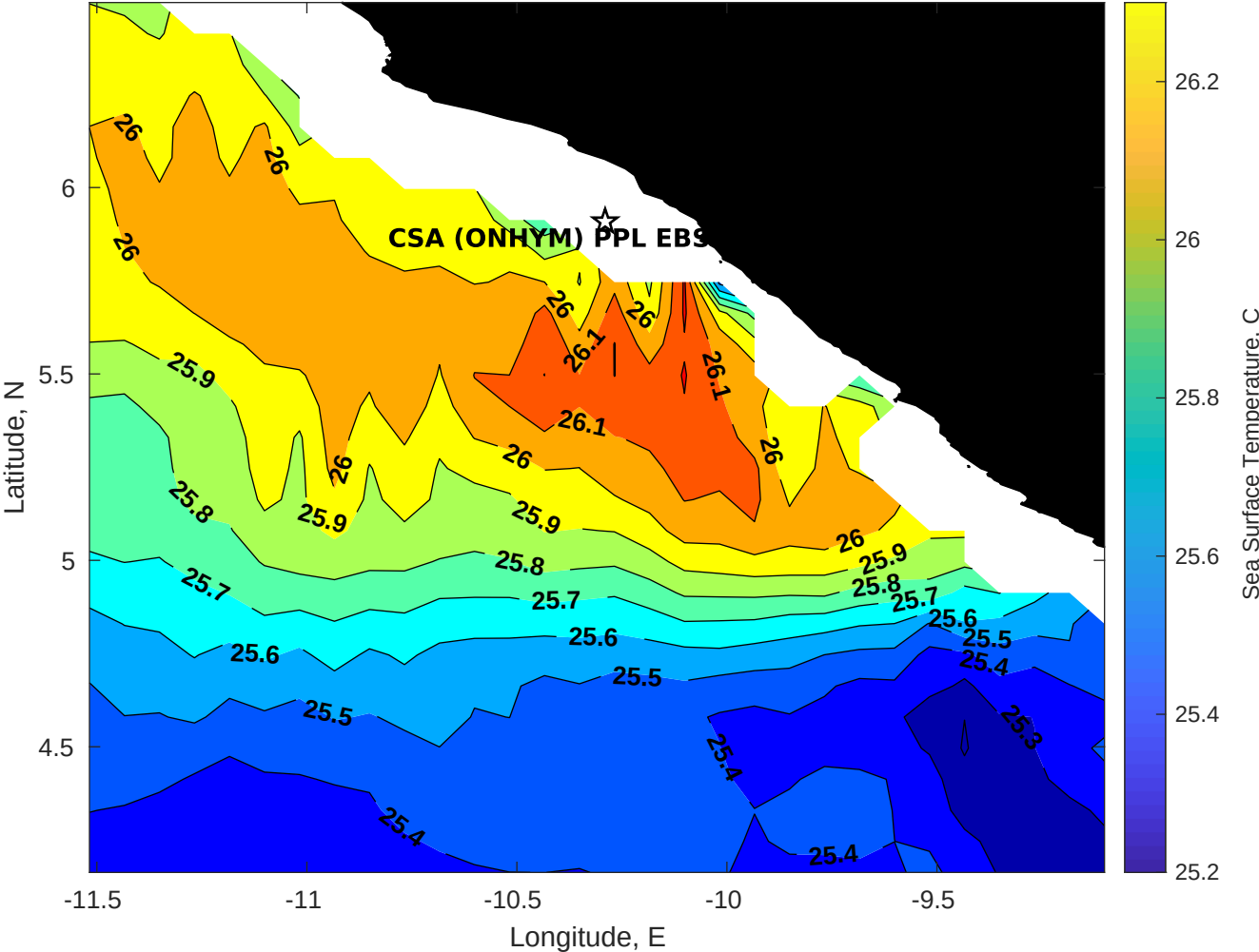
SST for CSA (ONHYM) PPL EBS - Liberia at 10-Aug-2025 00:00:00
