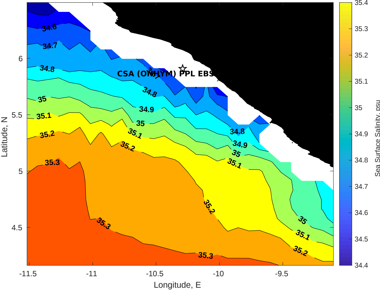
Surface Salinity for CSA (ONHYM) PPL EBS - Liberia at 10-Aug-2025 00:00:00
