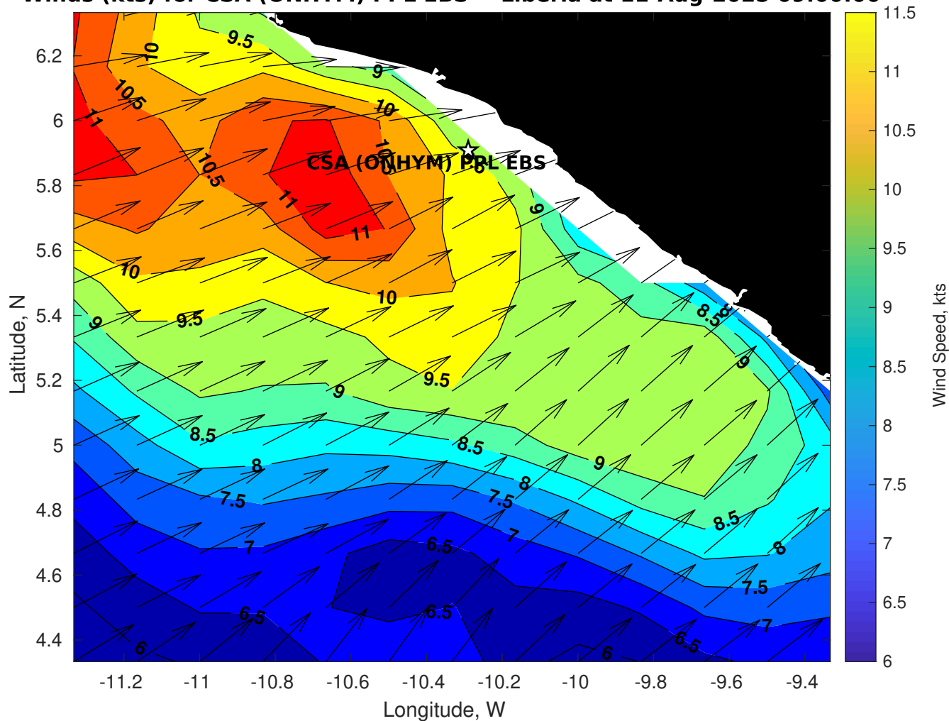
Winds (kts) for CSA (ONHYM) PPL EBS - Liberia at 11-Aug-2025 09:00:00
